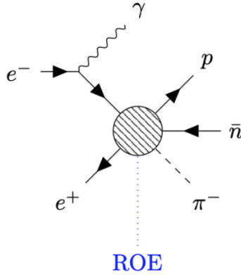
Figure 6.3: Feynman diagram of the channel of interest, with the Rest of Event ROE made of a variable amount of particles.
