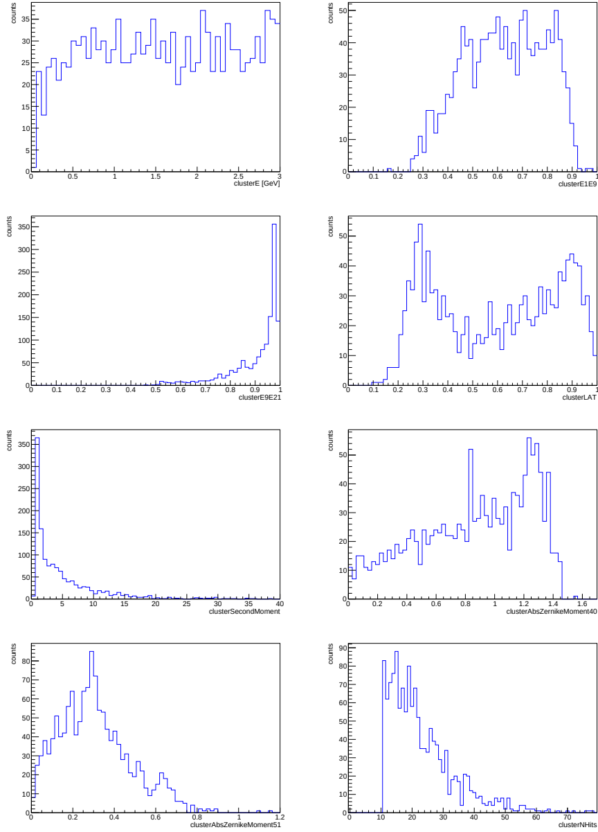
Figure 7.4: Reconstructed cluster variables for \bar{n} candidates, in NO ISR case. Data.
