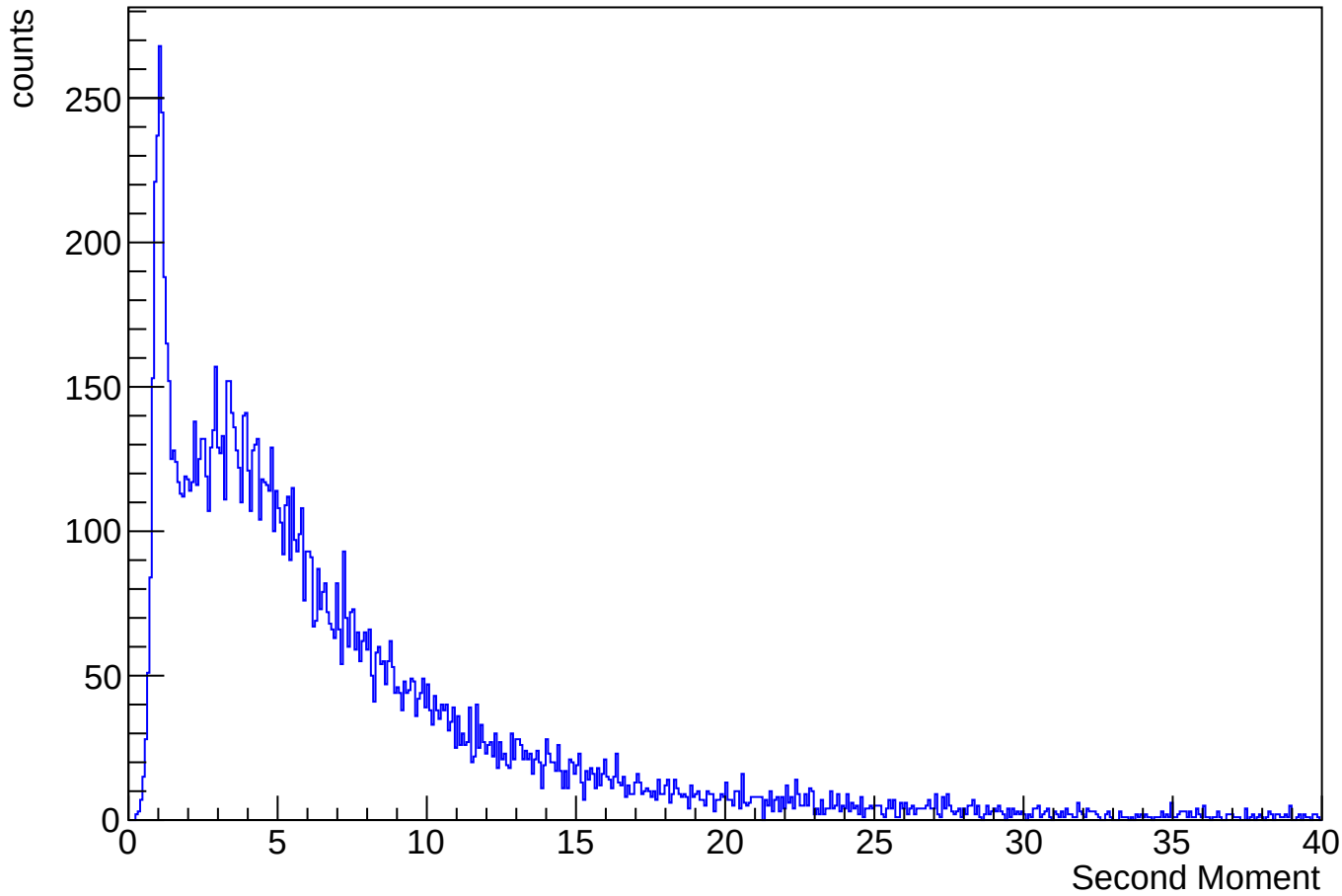
clusterSecondMoment
