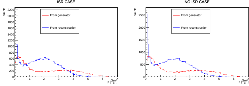
Figure 5.12: Momentum distribution of anti-neutron candidates, in both ISR (left) and NO ISR (right) cases.
