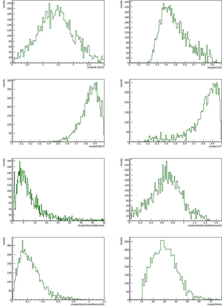
Figure 6.28: Reconstructed cluster variables for \bar{n} candidates after the application of the sidebands subtraction, in ISR case. \bar{q} cocktail.
