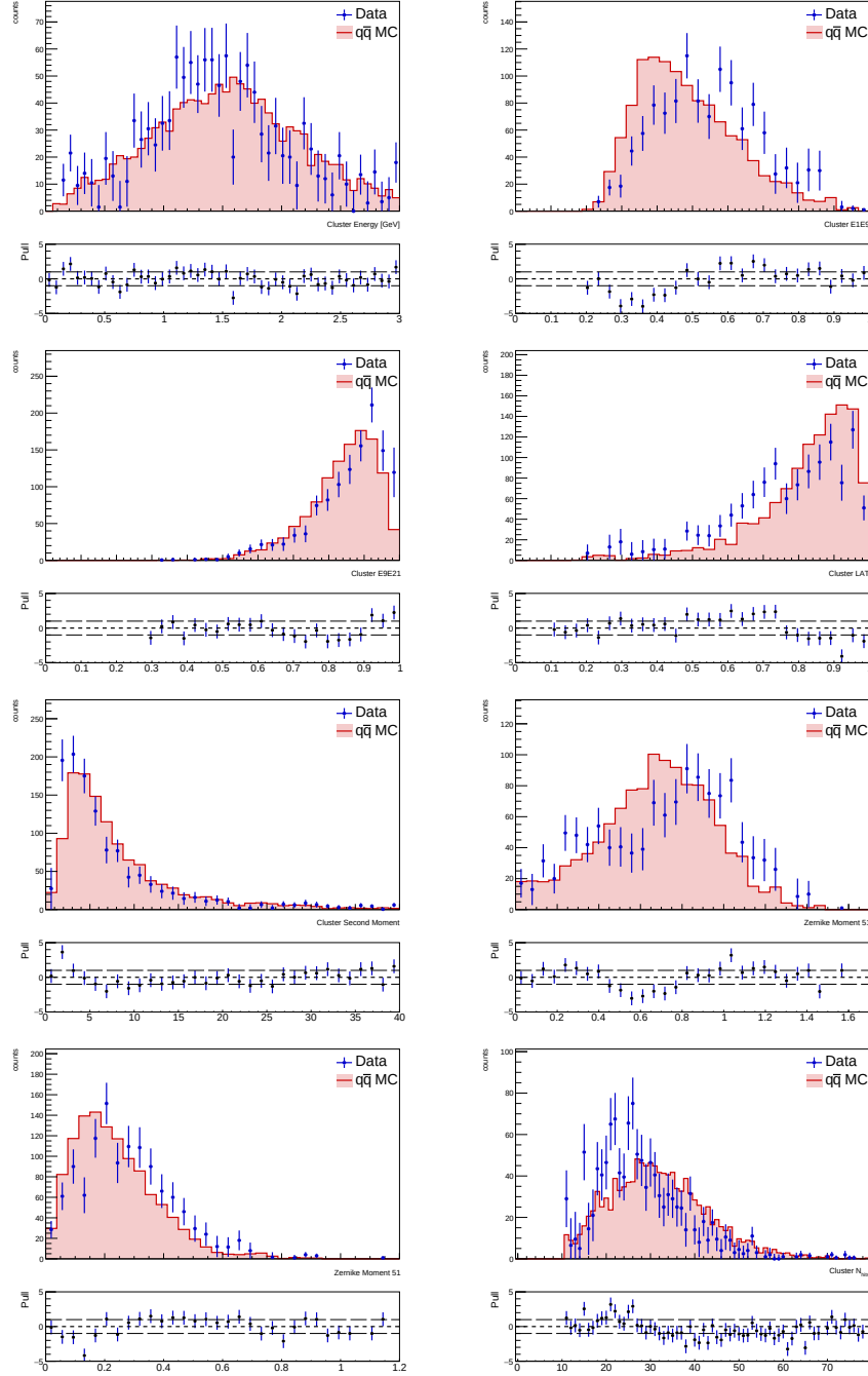
Figure 7.7: Data/MC agreement for reconstructed cluster variables for \bar{n} candidates, in ISR case. Sidebands technique applied. Signal region: [0.8, 1.4] GeV; sidebands region: [0.2, 0.8] \cup [1.4, 2.0] GeV.
