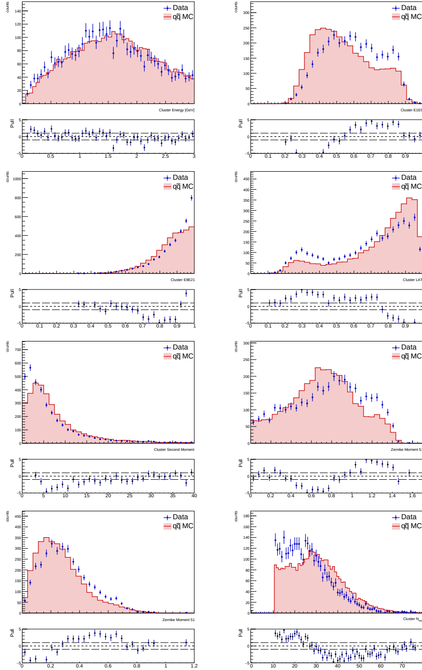
Figure 7.5: Data/MC agreement for reconstructed cluster variables for \bar{n} candidates, in ISR case.
