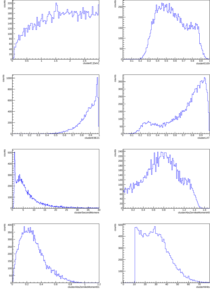
Figure 6.18: Cluster variables distributions for \bar{n} candidates in the recoil mass region [0, 2] \text{ GeV}/c^2 , in NO ISR case. q\bar{q} cocktail
