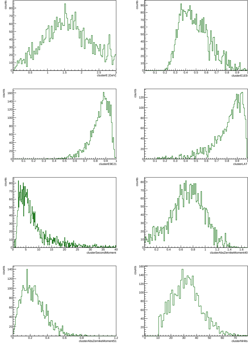
Figure 6.21: Reconstructed cluster variables for \bar{n} candidates, after the sidebands subtraction, in NO ISR case. q\bar{q} cocktail.
