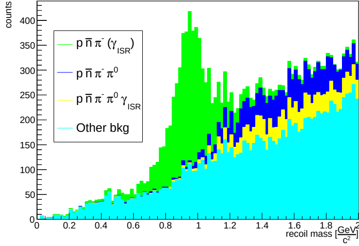
Figure 6.8: p, \pi^- recoil mass distribution in u\bar{u} Monte Carlo cocktail, displaying each stacked channels contribution, NO ISR case. Green: \pi^- \bar{n} p and \pi^- \bar{n} p \gamma_{ISR} channels. Blue: \pi^0 \pi^- \bar{n} p channel. Yellow: \pi^0 \pi^- \bar{n} p \gamma_{ISR} channel. Cyan: other channels.
