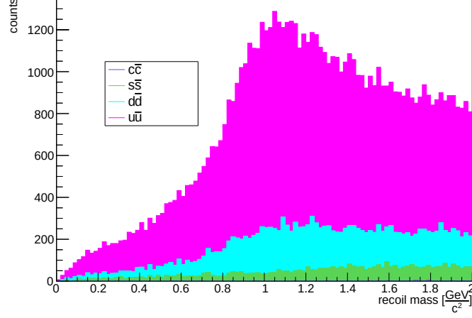
Figure 6.24: p, \pi^- recoil mass distribution in q\bar{q} Monte Carlo cocktail, displaying each stacked q\bar{q} component contribution, ISR case. (pink) u\bar{u} component; (light blue) d\bar{d} component; (green) s\bar{s} component; (blue) c\bar{c} component.
