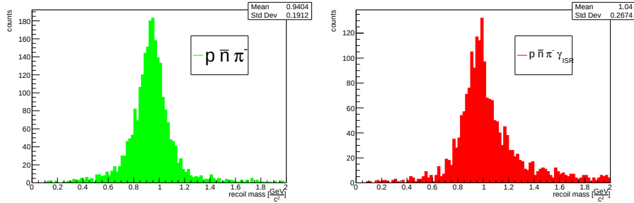
Figure 6.7: The p, \pi^- recoil mass for the channel with \pi^- \bar{n} p in the final state (green) and for the channel with \pi^- \bar{n} p \gamma_{ISR} in the final state (red).
