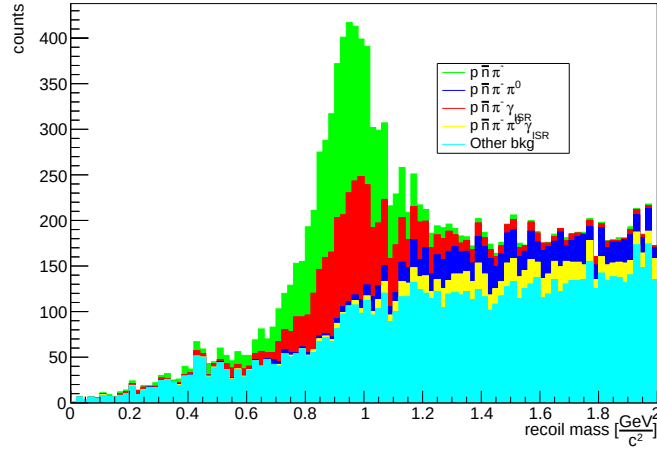
Figure 6.17: p, \pi^- recoil mass distribution in q\bar{q} Monte Carlo cocktail, displaying each stacked channel contribution, NO ISR case. Green: \pi^-\bar{n}p channel. Blue: \pi^0\pi^-\bar{n}p channel. Red: \pi^-\bar{n}p\gamma_{ISR} . Yellow: \pi^0\pi^-\bar{n}p\gamma_{ISR} channel. Cyan: other channels. \alpha < 10 rad cut is applied.
