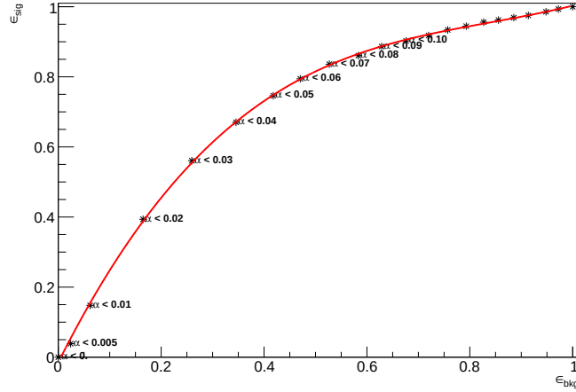
Figure 6.10: Receiver Operating Characteristic (ROC) curve constructed from the signal efficiency ( \epsilon_{sig} ) and the Background Efficiency ( \epsilon_{bkg} ), where each point corresponds to a different cut value on the \alpha angle. The labels are shown only for \alpha < 0.10 rad.
