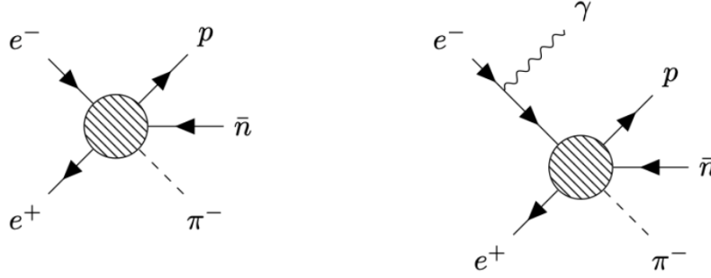
Figure 5.1: Feynman Diagrams of the channels of interest.
