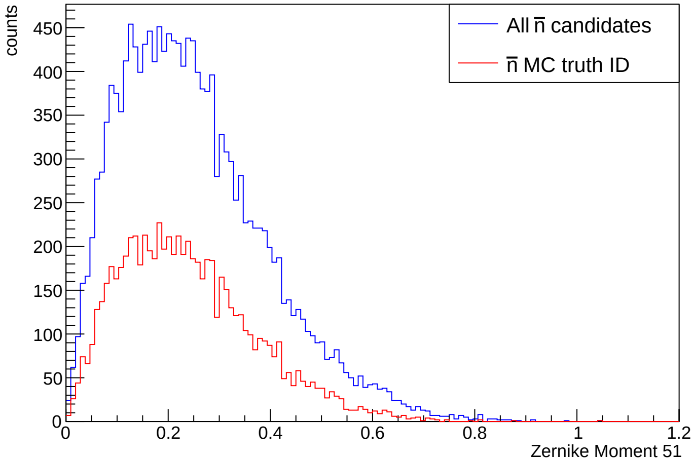
clusterAbsZernikeMoment51 with cut clusterNHits > 10
