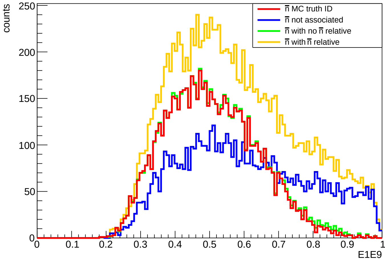
clusterE1E9
