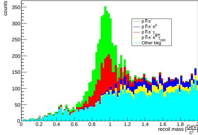
Figure 6.12: p, \pi^- recoil mass distribution, displaying each stacked channel contribution, NO ISR case. Green: \pi^- \bar{n} p channel. Blue: \pi^0 \pi^- \bar{n} p channel. Red: \pi^- \bar{n} p \gamma_{ISR} . Yellow: \pi^0 \pi^- \bar{n} p \gamma_{ISR} channel. Cyan: other channels. \alpha < 10 rad cut is applied.
