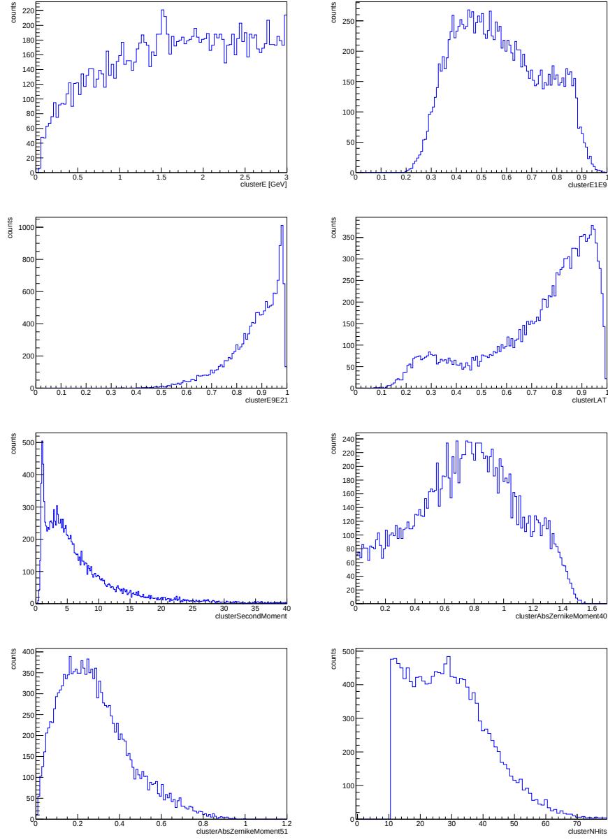
Figure 6.17: Cluster variables distributions for \bar{n} candidates in the recoil mass region [0, 2] \text{ GeV}/c^2 , in NO ISR case. q\bar{q} cocktail
