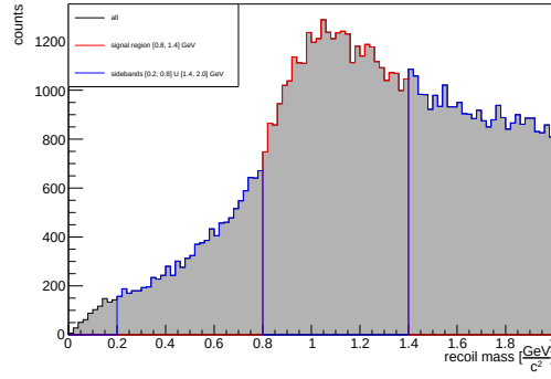
Figure 6.25: Recoil mass distribution (black), with the signal region (red) and the sidebands regions (blue), in the q\bar{q} Monte Carlo cocktail. ISR case.
