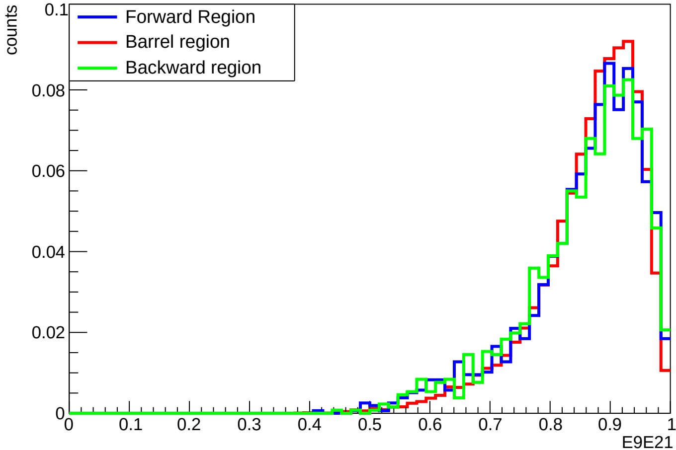
clusterE9E21 with cut clusterNHits > 10
