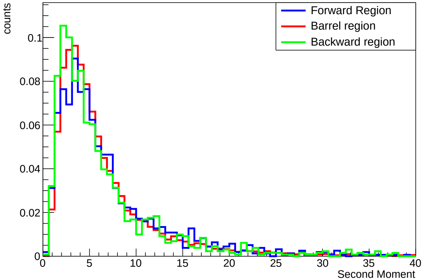
clusterSecondMoment with cut clusterNHits > 10
