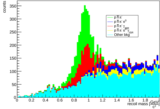
Figure 6.12: p, \pi^- recoil mass distribution, displaying each stacked component contribution, NO ISR case. Green: \pi^- \bar{n} p channel. Blue: \pi^0 \pi^- \bar{n} p channel. Red: \pi^- \bar{n} p \gamma_{ISR} . Yellow: \pi^0 \pi^- \bar{n} p \gamma_{ISR} channel. Cyan: other channels. \alpha < 10 rad cut is applied.
