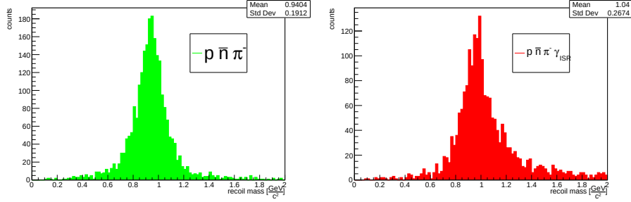
Figure 6.7: (green) p, \pi^- recoil mass and (red) p, \pi^-, \gamma_{ISR} recoil mas distributu in u\bar{u} Monte Carlo cocktail.
