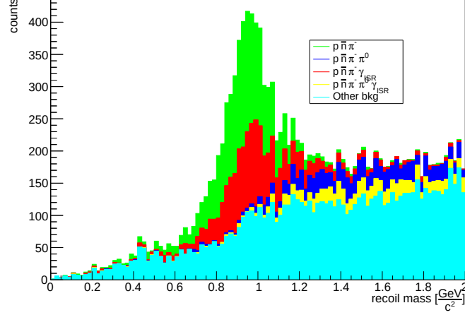
Figure 6.16: p, \pi^- recoil mass distribution in q\bar{q} Monte Carlo cocktail, displaying each stacked component contribution, NO ISR case. Green: \pi^- \bar{n} p channel. Blue: \pi^0 \pi^- \bar{n} p channel. Red: \pi^- \bar{n} p \gamma_{ISR} . Yellow: \pi^0 \pi^- \bar{n} p \gamma_{ISR} channel. Cyan: other channels. \alpha < 10 rad cut is applied.
