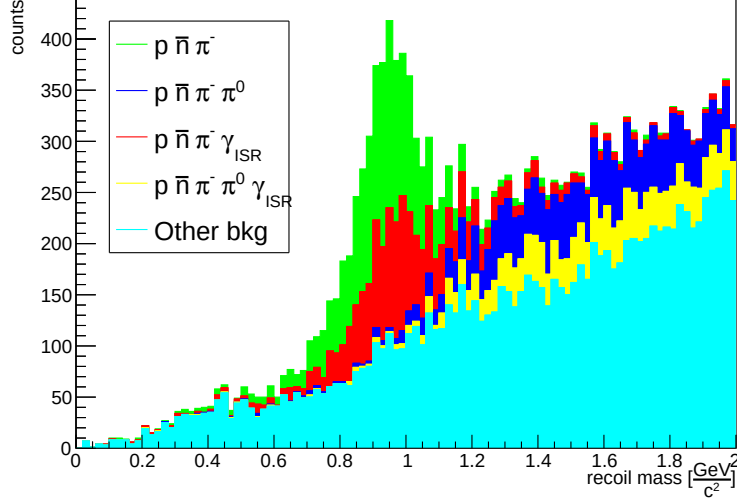
Figure 6.6: p, \pi^- recoil mass distribution in u\bar{u} Monte Carlo cocktail, displaying each stacked component contribution, NO ISR case. Green: \pi^-\bar{n}p channel. Blue: \pi^0\pi^-\bar{n}p channel. Red: \pi^-\bar{n}p\gamma_{ISR} . Yellow: \pi^0\pi^-\bar{n}p\gamma_{ISR} channel. Cyan: other channels.
