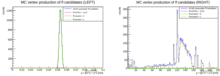
Figure 4.22: \bar{n} production vertex: (left) close to the IP (right) far from the IP
