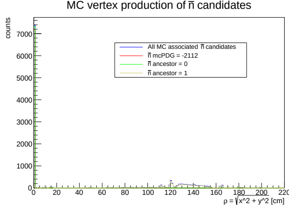
Figure 4.23: \bar{n} production vertex showing the IP peak is the main one
