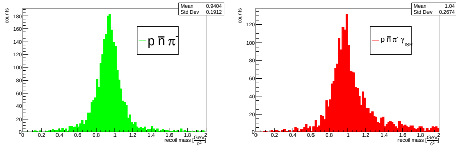
Figure 6.6: The p, \pi^- recoil mass for the channel with \pi^- \bar{n} p in the final state (green) and for the channel with \pi^- \bar{n} p \gamma_{ISR} in the final state (red).
