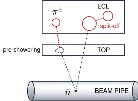
Figure 5.16: A representation displaying cluster split-off and pre-showering effects following \bar{n} annihilation. Figure not to scale.
