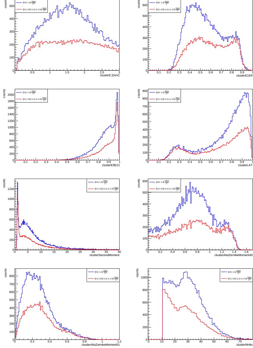
Figure 6.21: Comparison of reconstructed cluster variables for \bar{n} candidates in the signal region [0.8, 1.4] \text{ GeV}/c^2 (blue) with \bar{n} candidates in the sidebands region [0.2, 0.8] \cup [1.4, 2.0] \text{ GeV}/c^2 (red), in ISR case. A scaling factor of k = 0.5 has been applied to the cluster variables obtained from the sidebands regions. q\bar{q} cocktail.
