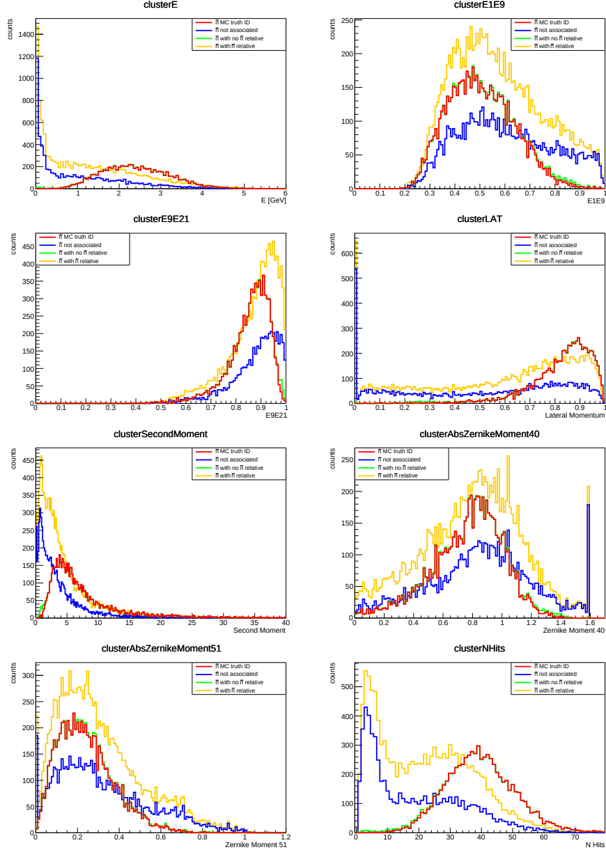
Figure 9.3: Comparison of reconstructed cluster variables for \bar{n} candidates with different ancestor selection (ISR case). Red: \bar{n} candidates associated with true \bar{n} by Monte Carlo matching; blue: \bar{n} candidates not associated with any particle (NaN); green: \bar{n} candidates without \bar{n} relatives; yellow: \bar{n} candidates with \bar{n} relative. The third contribution (green) is barely visible as it lies beneath the first distribution (red). ISR case.
