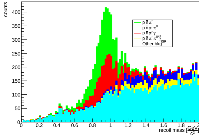
Figure 6.13: p, \pi^- recoil mass distribution in q\bar{q} Monte Carlo cocktail, displaying each stacked channel contribution, NO ISR case. Green: \pi^-\bar{n}p channel. Blue: \pi^0\pi^-\bar{n}p channel. Red: \pi^-\bar{n}p\gamma_{ISR} . Yellow: \pi^0\pi^-\bar{n}p\gamma_{ISR} channel. Cyan: other channels. \alpha < 10 rad cut is applied.
