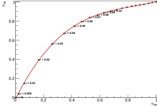
Figure 6.9: Receiver Operating Characteristic (ROC) curve constructed from the signal efficiency ( \epsilon_{sig} ) and the Background Efficiency ( \epsilon_{bkg} ), where each point corresponds to a different cut value on the \alpha angle. The labels are shown only for \alpha < 0.10 rad.
