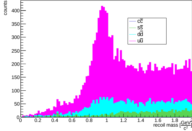
Figure 6.12: p, \pi^- recoil mass distribution in q\bar{q} Monte Carlo cocktail, displaying each stacked q\bar{q} component contribution, NO ISR case. (pink) u\bar{u} component; (cyan) d\bar{d} component; (green) s\bar{s} component; (blue) c\bar{c} component.
