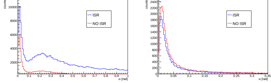
Figure 5.5: (a) \alpha distribution. (b) \alpha distribution after the rank selection.
