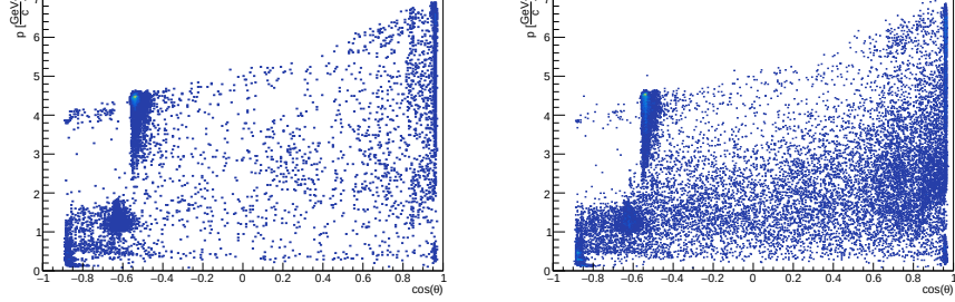
Figure 7.2: 2D \cos(\theta) vs momentum distribution in data. NO ISR case (left) and ISR case (right).
