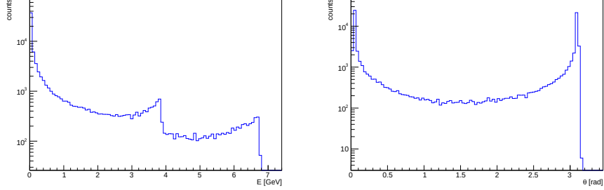
Figure 5.3: (left) ISR energy distribution. (right) ISR \theta distribution. Both distributions are shown on a logarithmic y -axis scale.
