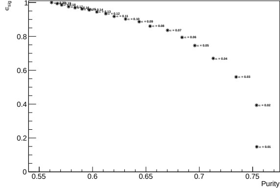
Figure 6.10: \epsilon_{sig} vs Purity curve for the u\bar{u} Monte Carlo cocktail.
