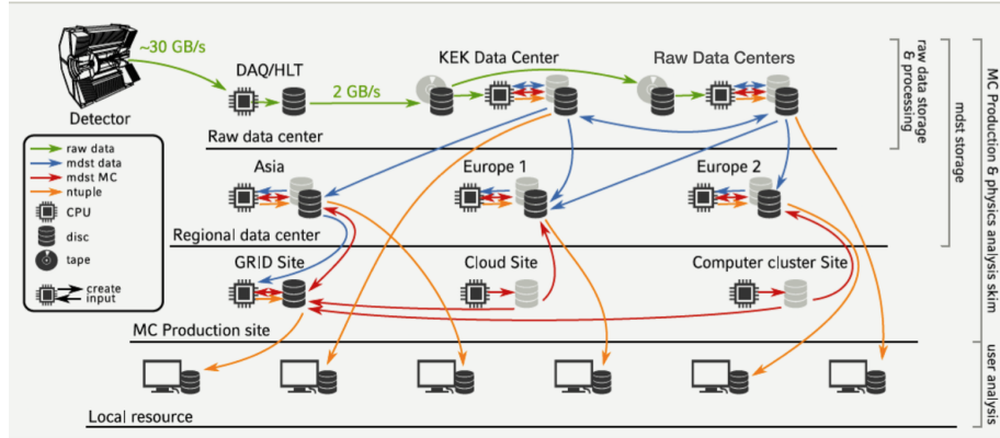
Figure 3.4: A scheme of the Belle II Distributed Computing sites.
