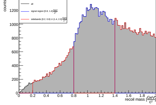
Figure 6.20: Recoil mass distribution (black), with the signal region (blue) and the sidebands regions (red), in the q\bar{q} Monte Carlo cocktail. ISR case.
