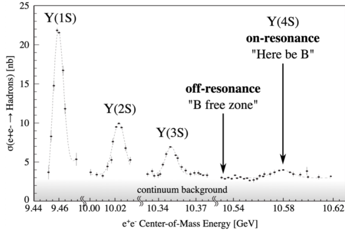
Figure 6.2: Cross section of e^+e^- \rightarrow \text{hadrons} , in the \Upsilon resonances energy region. The \Upsilon(1S) resonance is very narrow, while the \Upsilon(4S) one is broader and lower.
