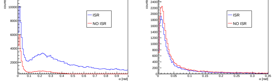
Figure 5.6: (a) \alpha distribution. (b) \alpha distribution after the rank selection.
