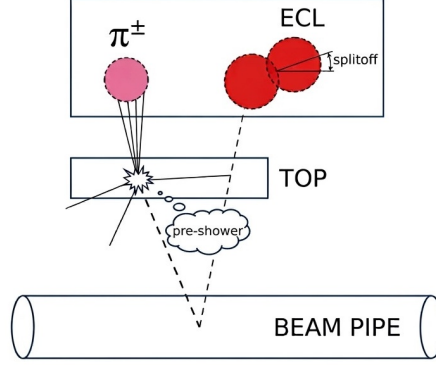
Figure 5.16: A representation displaying cluster split-off and pre-showering effects following \bar{n} annihilation.
