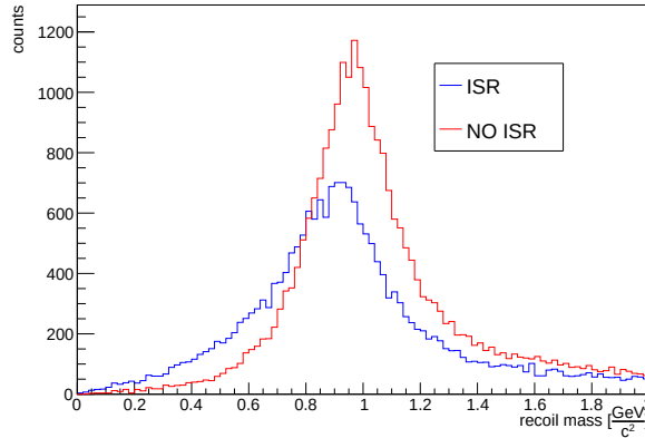
Figure 4.6: Recoil mass distribution, in both ISR and NO ISR cases
