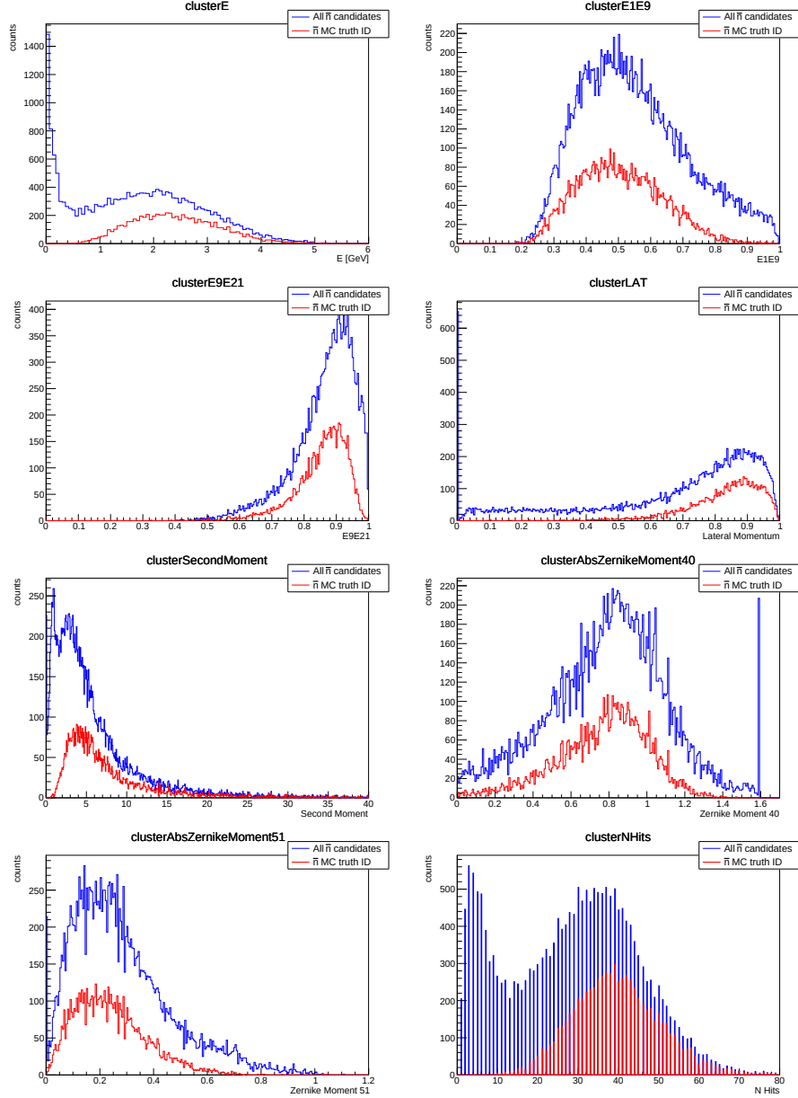
Figure 4.25: Comparison of reconstructed cluster variables for all \bar{n} candidates versus those associated with \bar{n} particles by Monte Carlo truth Monte Carlo PDG = -2112 (ISR case). The selection is performed using the Monte Carlo PDG code (-2112), as previously discussed
