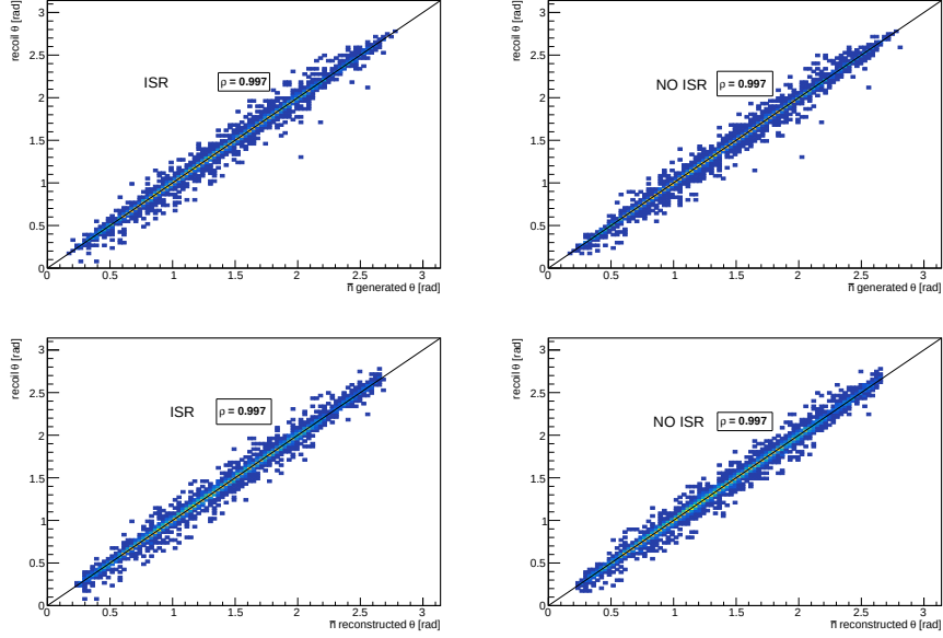
Figure 4.12: \theta correlation distribution between recoil system and anti-neutron candidate, in both reconstructed and generated case. Linear correlation coefficient \rho truncated to three decimal places
