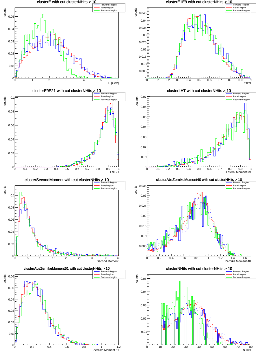
Figure 4.32: Comparison of reconstructed cluster variables for all \bar{n} candidates in different ECL regions. The distributions are normalized to unit value
