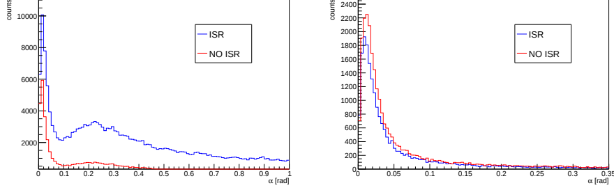
Figure 4.4: (a) \alpha distribution (b) \alpha distribution after the rank selection
