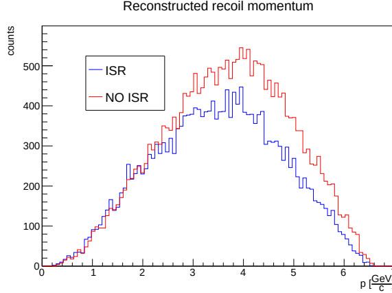
Figure 4.9: Reconstructed momentum distribution of the recoil system, in both ISR and NO ISR cases
