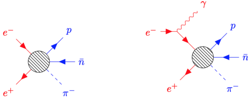
Figure 4.2: Feynman diagram of the channel of interest. Phokhara handles the initial hard photon emission (red), while EvtGen simulates the decay to final-state particles (blue).
