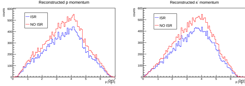
Figure 4.7: Reconstructed momentum distribution of proton and pion, in both ISR and NO ISR cases
