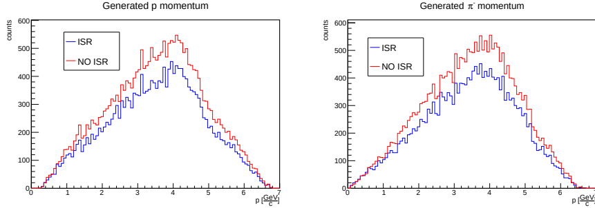
Figure 4.8: Generated momentum distribution of proton and pion, in both ISR and NO ISR cases
