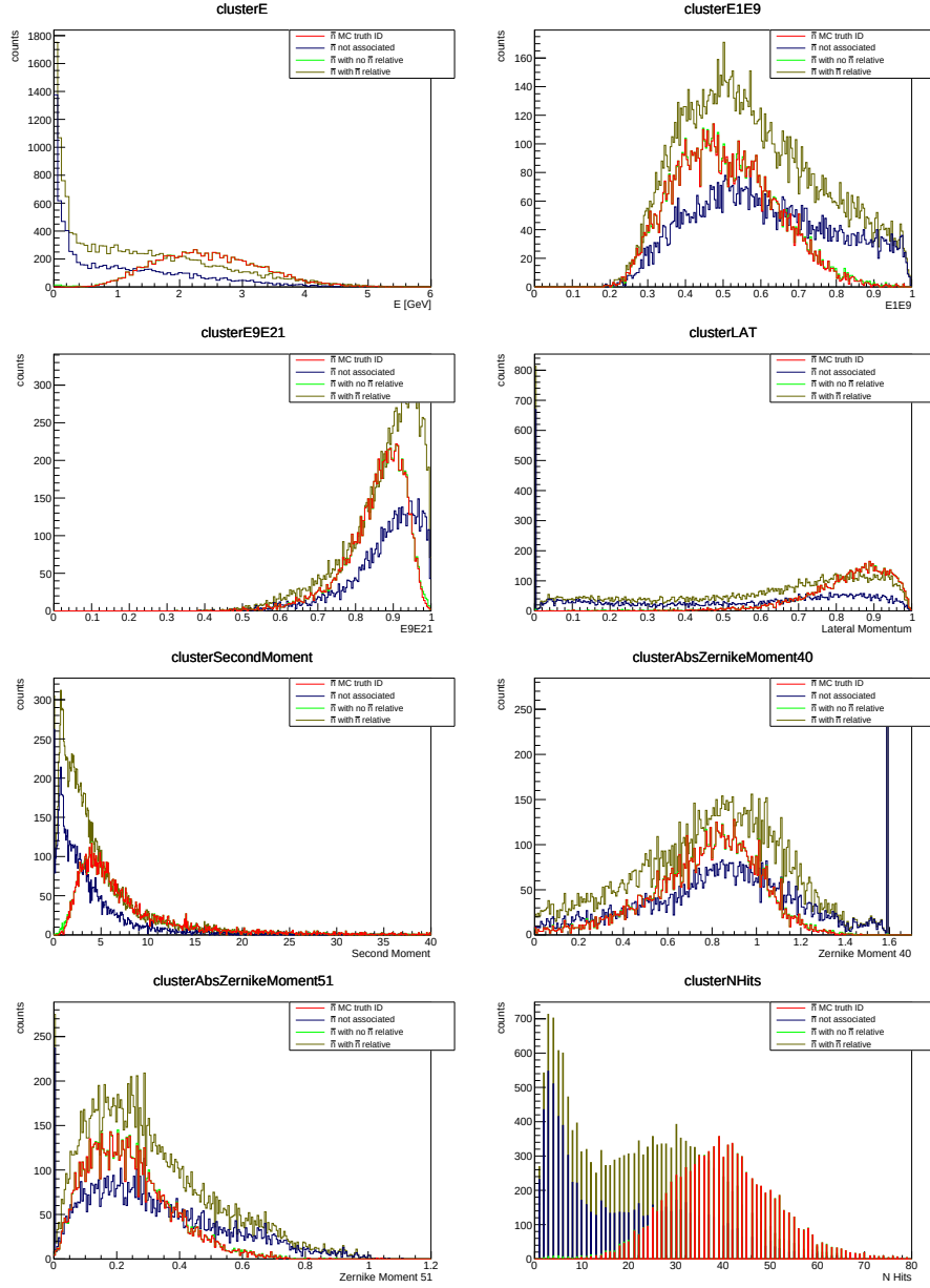
Figure 4.28: Comparison of reconstructed cluster variables for \bar{n} candidates with different ancestor selection (NO ISR case)
