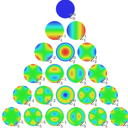
Figure 4.24: Zernike Polynomials representation. Moments Z_4^0 and Z_5^1 are widely discussed in this thesis
