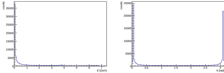
Figure 4.5: (a) ISR energy distribution (b) ISR \theta distribution
