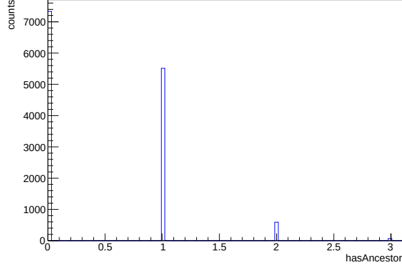
Figure 4.16: Distribution of the ancestry kinship degree of anti-neutron candidates with an anti-neutron present in their ancestry chain
