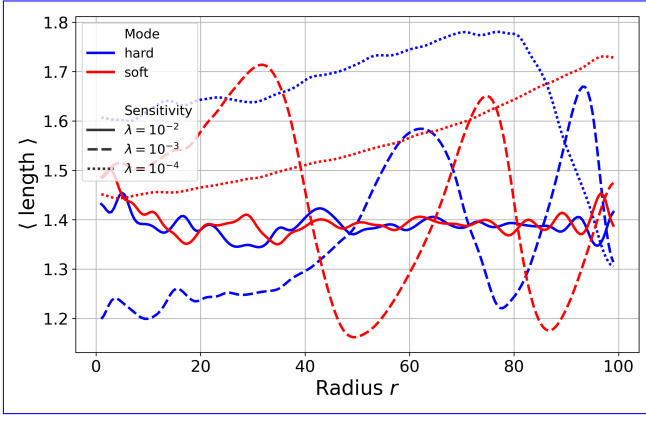
Figure 5: The average length of the cells at increasing radial distance from the center, for a colony of length R \approx 100 . The hard and soft models show similar qualitative patterns for each \lambda , but differ significantly in the location of the “peaks”.
