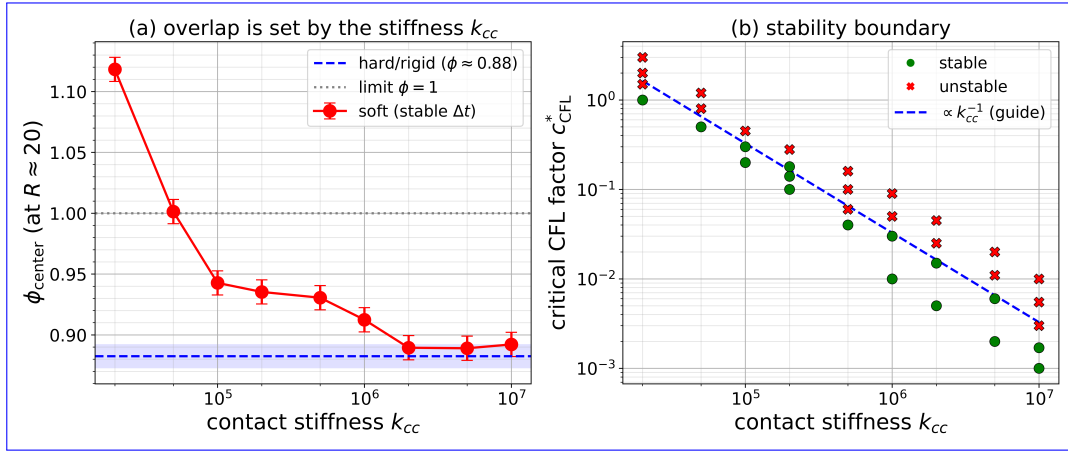
Figure 6: The soft model's excess central packing results from the contact stiffness, but reducing this to produce similar packing fractions as the hard model requires a lower c_{\text{CFL}}^* and hence smaller step-size. (a) The overlap is set by the stiffness: increasing k_{cc} , each run at a step-size small enough for stability, drives the center packing fraction \phi_{\text{center}} = \phi(6) = \frac{A_{\text{cells}(6)}}{A_{\text{total}(6)}} (compared at R \approx 20, \lambda = 10^{-4} ) toward the rigid packing of the hard model (dashed). (b) The stiffness cannot be increased for free. The critical CFL factor c_{\text{CFL}}^* separating stable (green) from unstable (red) runs scales at approximately k_{cc}^{-1} . A run is classified as unstable if any cell's single-step displacement exceeds half its length. A soft model (large k_{cc} ) that closely reproduces the hard model therefore requires a prohibitively small step-size and thus a higher cost.
