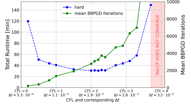
Figure 19: Total runtime to reach colony radius 100 versus CFL factor on 112 cores (each point is an independent run). A U-shaped trend emerges: small CFL values increase timestep count, while large values raise BBPGD iterations per step. The annotated \Delta t denotes the mean step-size. The red region indicates CFL values where the solver fails to converge.
