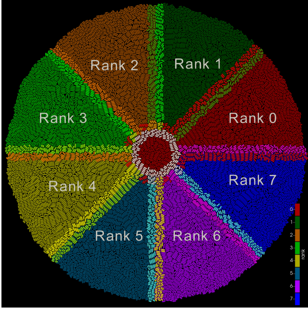
Figure 16: Domain decomposition for 8 MPI ranks showing evenly spaced angular sectors of a colony with radius 50. Each rank owns one angular sector. Ghost particles at rank boundaries are shown in brighter colors.
