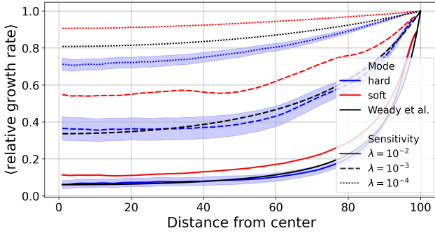
Figure 11: Radial relative growth rate profiles ( e^{-\lambda\sigma} ) for both models. Cells in the soft model grow significantly faster than those in the hard model across most of the colony, particularly at low stress-sensitivity values. At high stress-sensitivity ( \lambda = 10^{-2} ), growth is strongly suppressed in the interior of both models, with only cells at the colony edge actively dividing. The black lines indicate the theoretical growth rates derived from the continuum model in [35].
