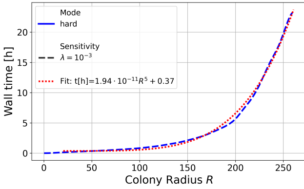
Figure 21: Wall time as a function of colony radius. The wall time roughly follows T_{\text{wall}} [\text{h}] \approx 1.94 \cdot 10^{-11} R^5 + 0.37 .
