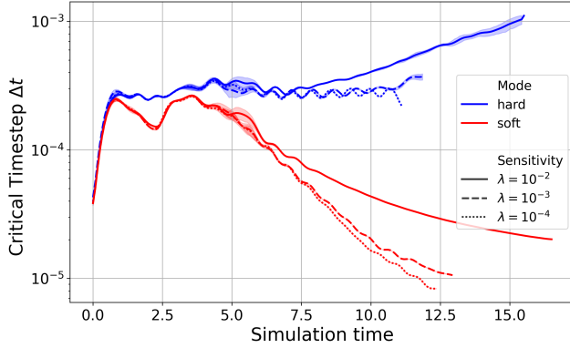
Figure 18: Adaptive step-size \Delta t over simulation time for both models. During early growth, \Delta t is similar and set by cell growth velocities. As the colony densifies, the soft model becomes collision-dominated, with large overlaps increasing velocities and reducing \Delta t to \approx 10^{-5} . The hard model avoids this, maintaining stable or increasing \Delta t due to constraint-based separation and reduced interior growth.
