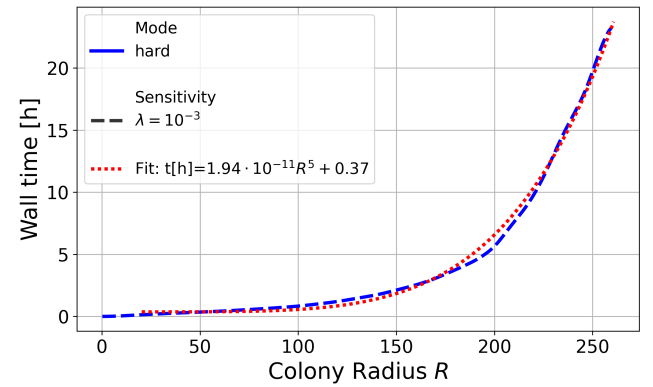
Figure 21: Wall time as a function of colony radius. The wall time roughly follows T_{\text{wall}} [\text{h}] \approx 1.94 \cdot 10^{-11} R^5 + 0.37 .
