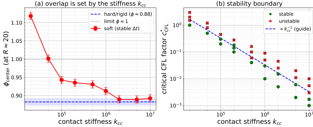
Figure 6: The soft model's excess central packing results from the contact stiffness, but reducing this to produce similar packing fractions as the hard model requires a lower c_{\text{CFL}}^* and hence smaller step-size. (a) The overlap is set by the stiffness: increasing k_{cc} , each run at a step-size small enough for stability, drives the center packing fraction \phi_{\text{center}} = \phi(6) = \frac{A_{\text{cells}}(6)}{A_{\text{total}}(6)} (compared at R \approx 20, \lambda = 10^{-4} ) toward the rigid packing of the hard model (dashed). (b) The stiffness cannot be increased for free. The critical CFL factor c_{\text{CFL}}^* separating stable (green) from unstable (red) runs scales at approximately k_{cc}^{-1} . A run is classified as unstable if any cell's single-step displacement exceeds half its length. A soft model (large k_{cc} ) that closely reproduces the hard model therefore requires a prohibitively small step-size and thus a higher cost.
