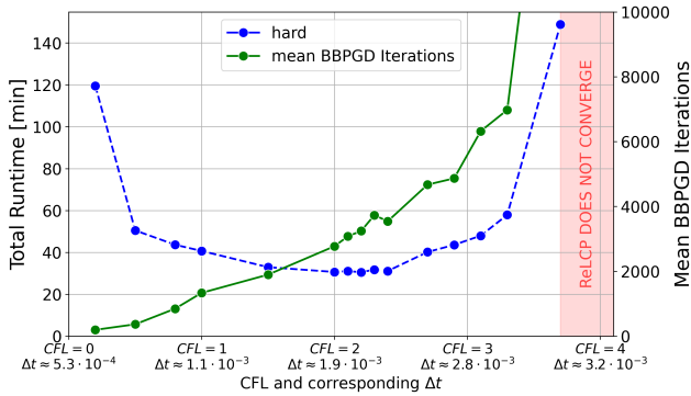
Figure 19: Total runtime to reach colony radius 100 versus CFL factor on 112 cores (each point is an independent run). A U-shaped trend emerges: small CFL values increase timestep count, while large values raise BBPGD iterations per step. The annotated \Delta t denotes the mean step-size. The red region indicates CFL values where the solver fails to converge.
