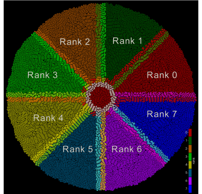
Figure 16: Domain decomposition for 8 MPI ranks showing evenly spaced angular sectors of a colony with radius 50. Each rank owns one angular sector. Ghost particles at rank boundaries are shown in brighter colors.
