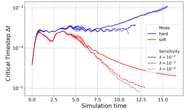
Figure 18: Adaptive step-size \Delta t over simulation time for both models. During early growth, \Delta t is similar and set by cell growth velocities. As the colony densifies, the soft model becomes collision-dominated, with large overlaps increasing velocities and reducing \Delta t to \approx 10^{-5} . The hard model avoids this, maintaining stable or increasing \Delta t due to constraint-based separation and reduced interior growth.
