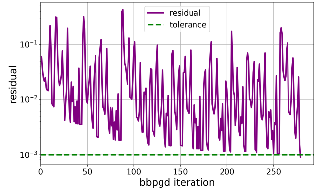
(b) BBPGD residuals over iterations for a single timestep. The solver converges to tolerance \epsilon = 10^{-3} within approximately 280 iterations, showing highly oscillatory behavior. The residual directly represents the current maximum overlap between any two cells in the colony.
