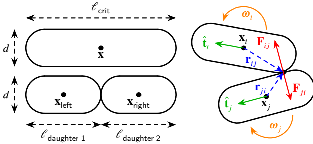
Figure 2: Spherocylinder cell model. Cells are modeled as 3D spherocylinders; the diagram shows a 2D schematic view. Contact forces \mathbf{F}_{ij} (red) and lever arms \mathbf{r}_{ij} (dashed blue) generate torques causing angular motion \omega (orange), and also produce translational displacements of the cells. The longitudinal axis \hat{\mathbf{t}}_i (green) defines the direction along which stress is projected. Cell division occurs when a cell reaches critical length \ell_{\text{crit}} .
