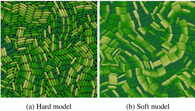
Figure 6: Close-up comparison of cell packing in the colony center for both collision models. The hard model (a) maintains near-optimal packing, while the soft model (b) exhibits significant overlap and overcrowding.
