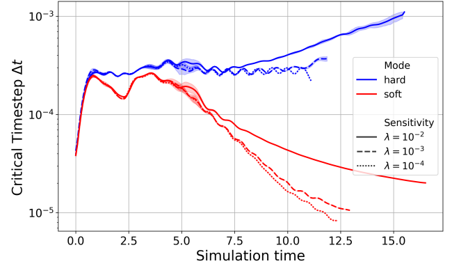
Figure 17: Adaptive step-size \Delta t over simulation time for both models. During early growth, \Delta t is similar and set by cell growth velocities. As the colony densifies, the soft model becomes collision-dominated, with large overlaps increasing velocities and reducing \Delta t to \approx 10^{-5} . The hard model avoids this, maintaining stable or increasing \Delta t due to constraint-based separation and reduced interior growth.
