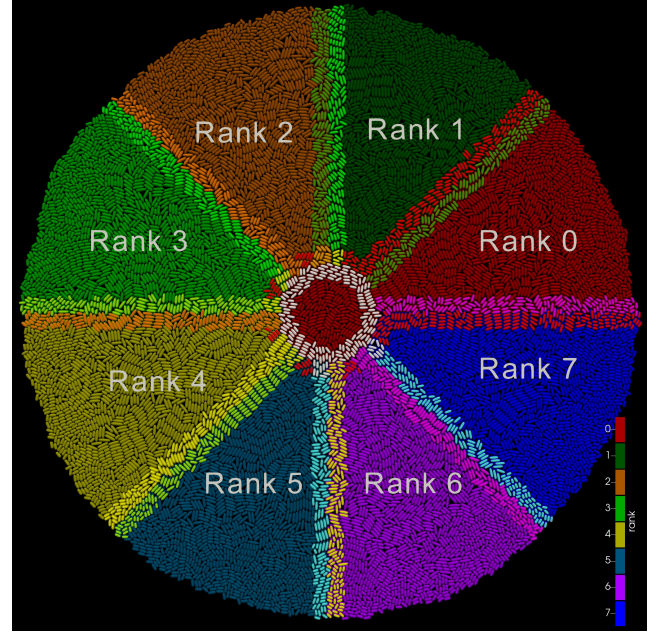
Figure 15: Domain decomposition for 8 MPI ranks showing evenly spaced angular sectors of a colony with radius 50. Each rank owns one angular sector. Ghost particles at rank boundaries are shown in brighter colors.
