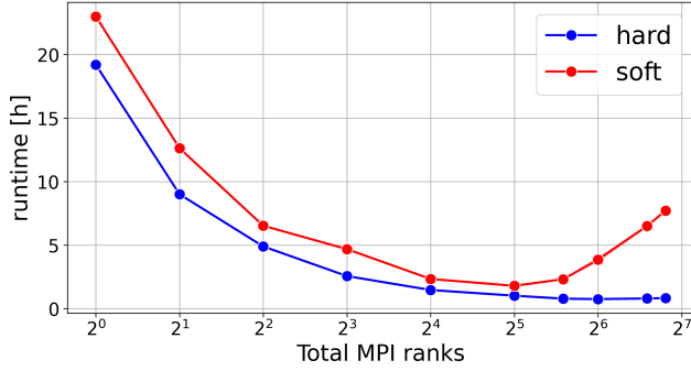
(a) Runtime to reach colony radius of 100 versus MPI ranks. The hard model is consistently faster, with the performance gap widening at high core counts.
