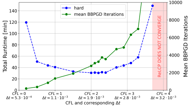
Figure 18: Total runtime to reach colony radius 100 versus CFL factor on 112 cores (each point is an independent run). A U-shaped trend emerges: small CFL values increase timestep count, while large values raise BBPGD iterations per step. The annotated \Delta t denotes the mean step-size. The red region indicates CFL values where the solver fails to converge.
