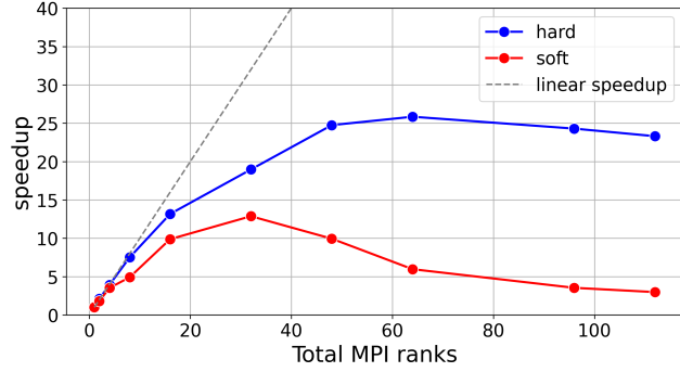
(b) Speedup versus MPI ranks. The hard and soft models scale reasonably up to 64 and 32 ranks, respectively.
