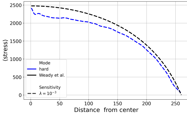
(c) Radial stress profile of the hard model at R = 260 . The simulated stress closely follows the analytical prediction from [33], confirming global mechanical balance across the colony.
