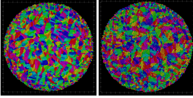
(a) Soft model with \lambda = 10^{-2} at colony radius R \approx 50 . (b) Hard model with \lambda = 10^{-2} at colony radius R \approx 50 .
