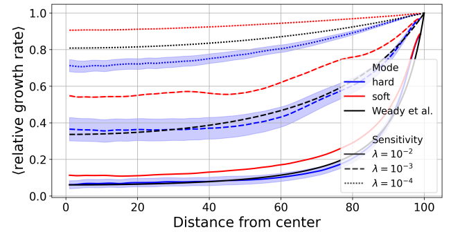
Figure 10: Radial relative growth rate profiles ( e^{-\lambda\sigma} ) for both models. Cells in the soft model grow significantly faster than those in the hard model across most of the colony, particularly at low stress-sensitivity values. At high stress-sensitivity ( \lambda = 10^{-2} ), growth is strongly suppressed in the interior of both models, with only cells at the colony edge actively dividing. The black lines indicate the theoretical growth rates derived from the continuum model in [32].
