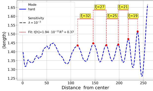
(b) Radial distribution of the average cell length for the hard model at R = 260 . The oscillatory pattern has a characteristic ring spacing of \xi \approx 25 , consistent with the radial ring spacing visible in Figure A1.
