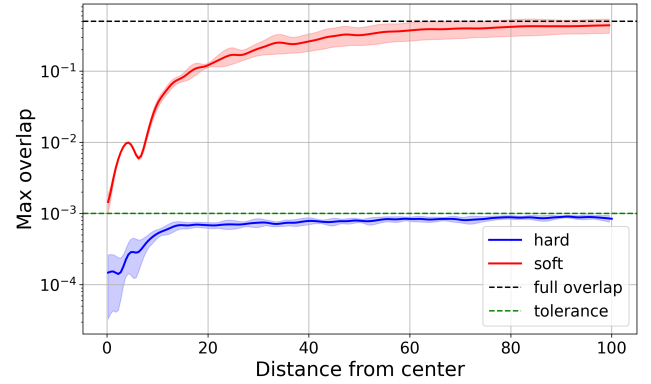
(b) Maximum cell overlap as a function of distance from the colony center. The hard model remains uniformly near solver tolerance \varepsilon = 10^{-3} , whereas the soft model exhibits substantially elevated overlap at all radial positions, with values near the colony boundary approaching full cell overlap.
