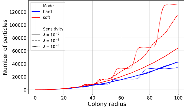
(a) Number of cells required to reach a given colony radius. The soft model requires substantially more cells, particularly at low stress-sensitivity ( \lambda = 10^{-4} ).
