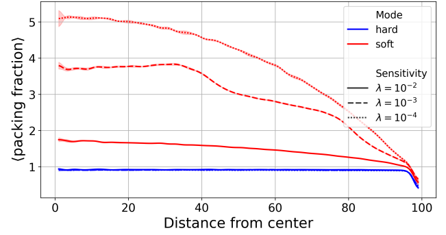
(a) Radial packing fraction profiles ( \phi = \frac{A_{\text{cells}}}{A_{\text{total}}} ) for both models. Here, A_{\text{cells}} denotes the total area occupied by cells within a spatial bin of width 2 at distance r from the colony center, and A_{\text{total}} is the corresponding annular bin area. The hard model maintains nearly optimal packing, while the soft model exhibits elevated fractions in the colony center, particularly at low stress-sensitivity ( \lambda = 10^{-4} ).
