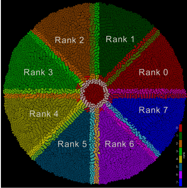
Figure 12: Domain decomposition for 8 MPI ranks showing evenly spaced angular sectors of a colony with radius 50. Each rank owns one angular sector. Ghost particles at rank boundaries are shown in brighter colors.
