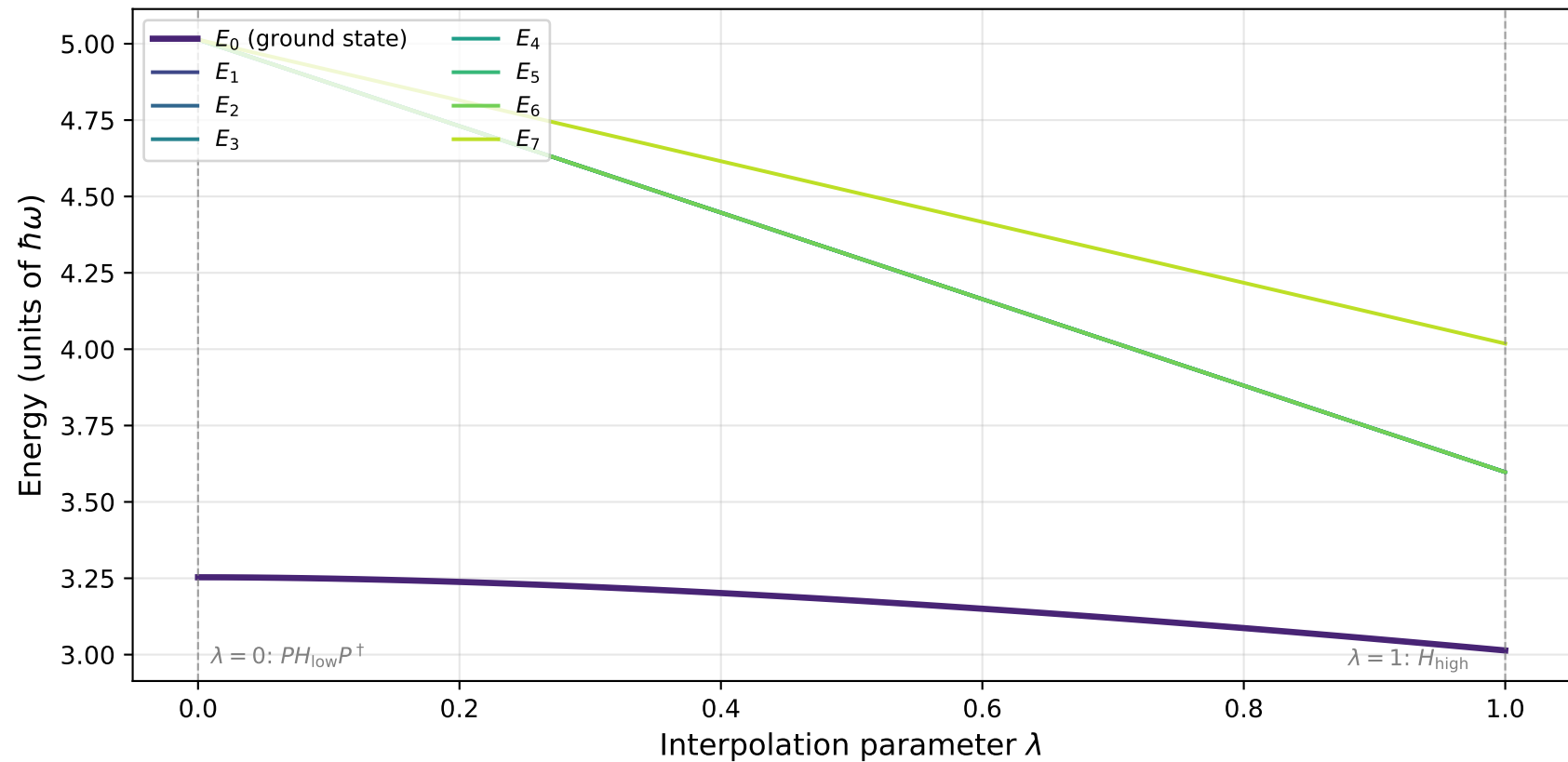
N = 2 quantum dot, K_{\text{low}} = 2 , \hbar\omega = 1
