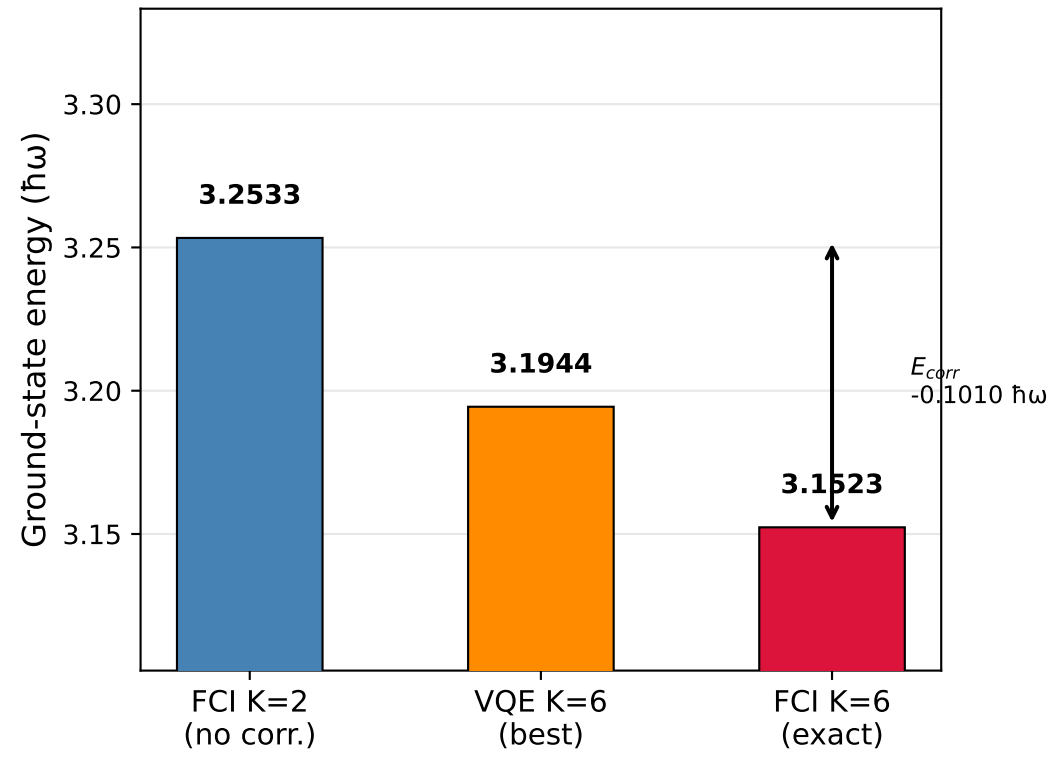
K=2 vs K=6: correlation energy N = 2 , \hbar\omega = 1
