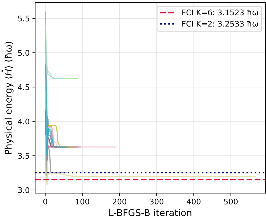
VQE K=6 energy convergence 16 random starts, 2-stage NM→L-BFGS-B
