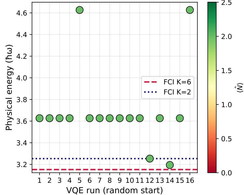
Final VQE energies per run coloured by \langle \hat{N} \rangle
