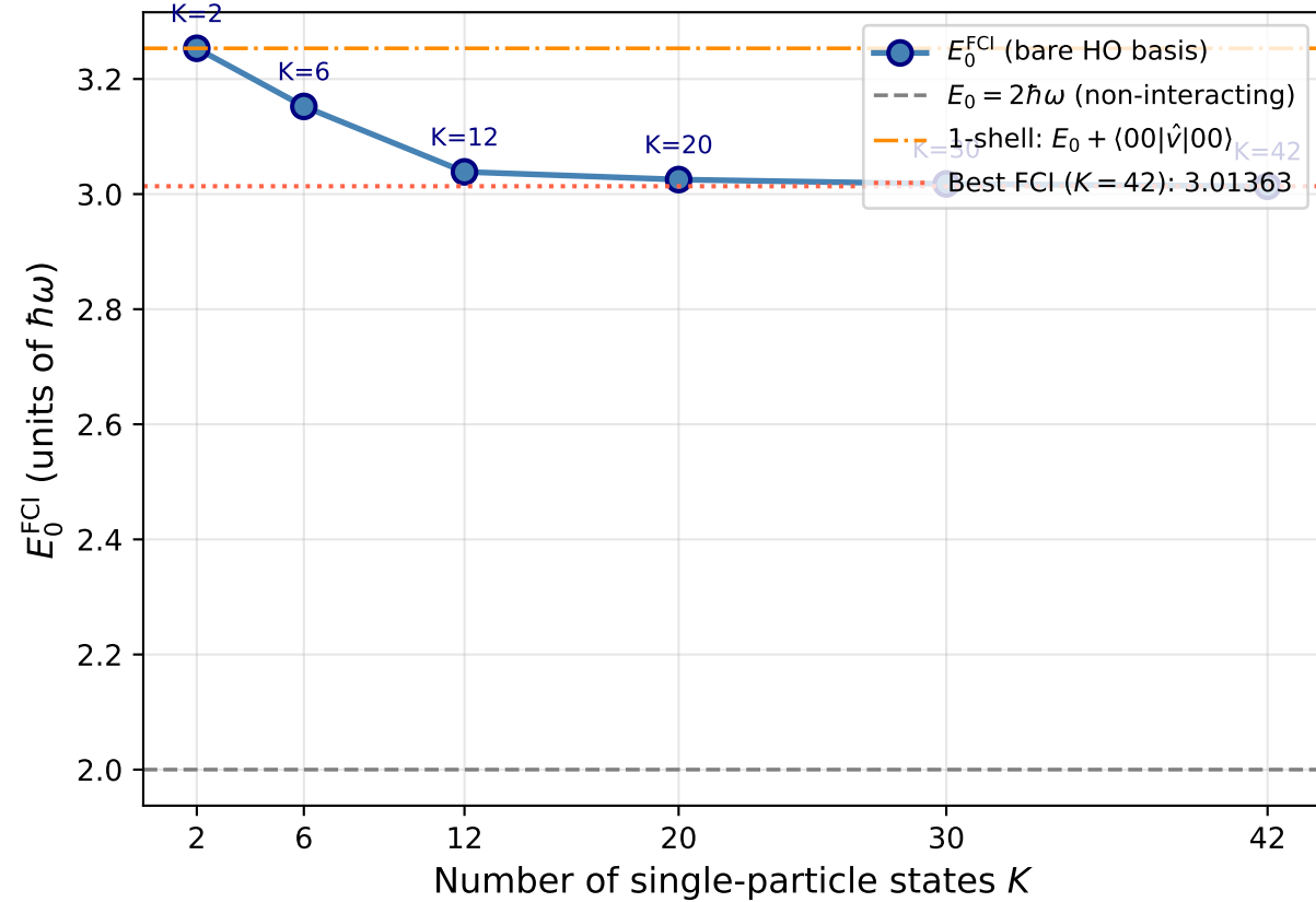
FCI ground-state energy vs basis size N = 2 electrons, bare HO basis, \hbar\omega = 1
