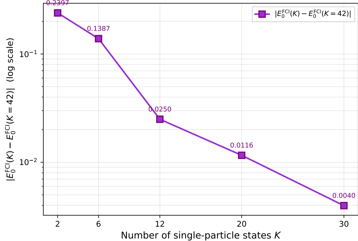
FCI convergence to K = 42 result N = 2 , bare HO basis, \hbar\omega = 1
