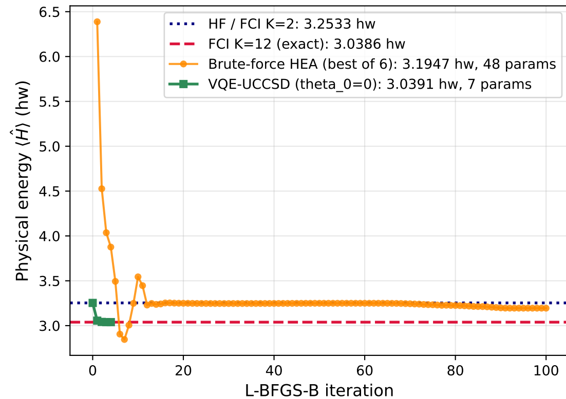
VQE on the K=12 quantum dot (N=2 electrons, \hbar\omega=1 ): HEA vs UCCSD
