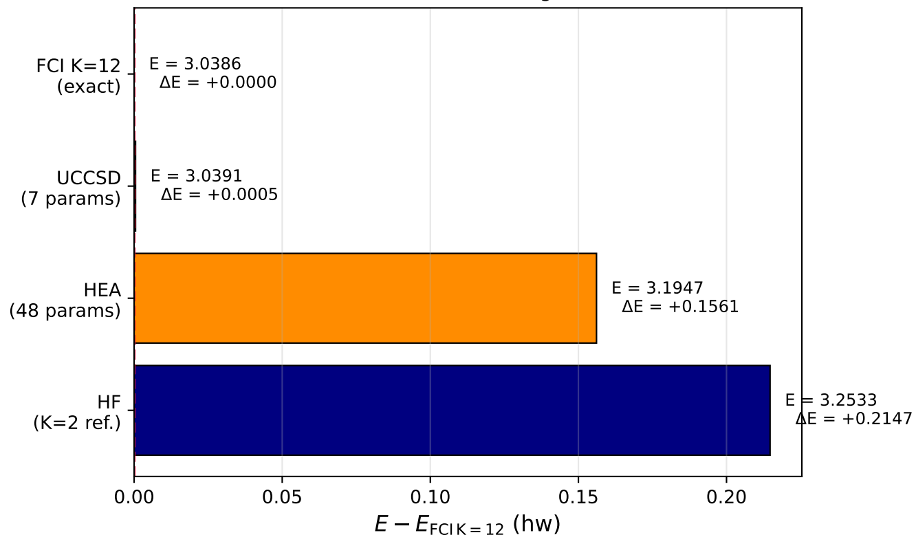
Distance from exact K=12 ground state
