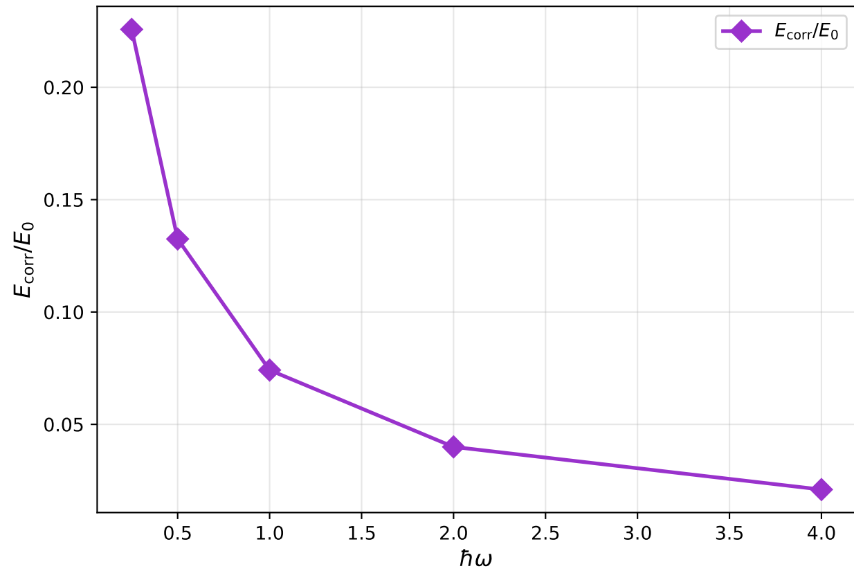
Relative correlation energy E_{\text{corr}} = E_{\text{HF}} - E_{\text{FCI}}, K = 42
