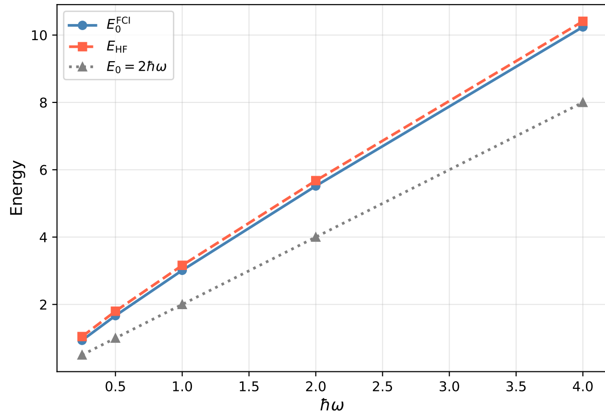
FCI and HF energies vs \hbar\omega N = 2, K = 42
