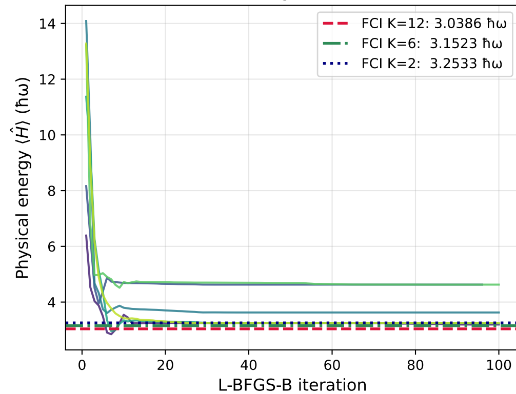
VQE K=12 convergence 6 starts, 2-stage NM→L-BFGS-B
