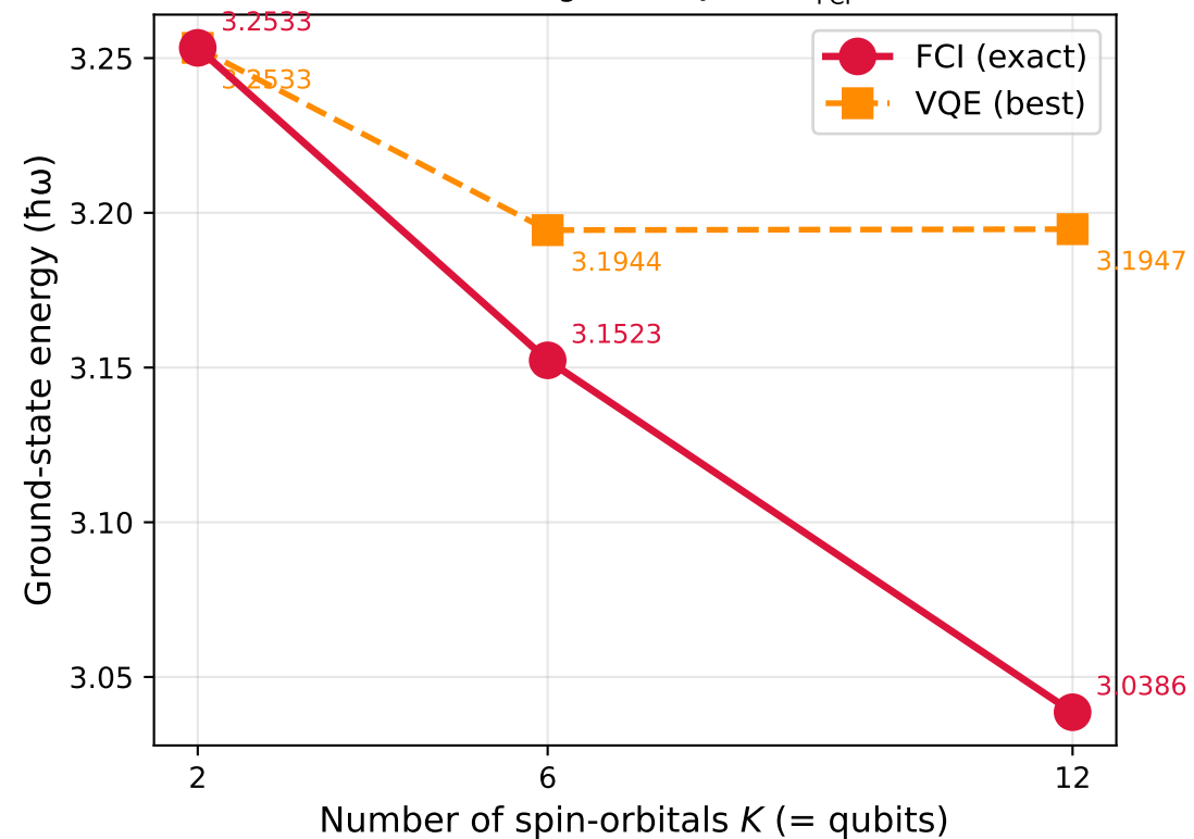
K-convergence: E_0(K) \rightarrow E_{\text{FCI}}^\infty
