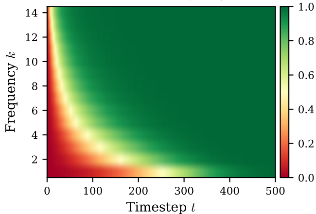
White DDPM: R^2(t)
