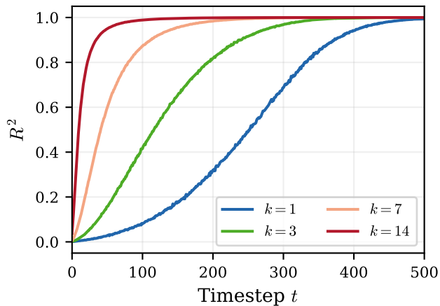
White DDPM: R^2(t)
