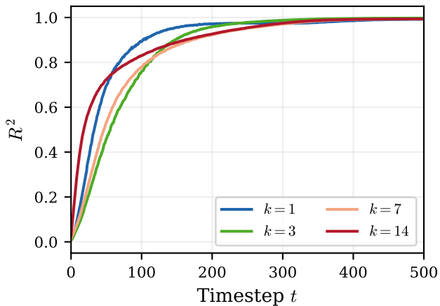
Flicker-DDPM: R^2(t)
