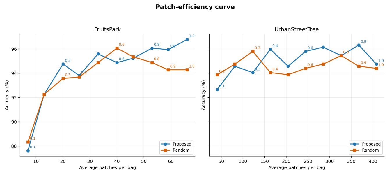
FIGURE 10. Patch-efficiency curves comparing the proposed TBS-DepthAug configuration with random sparse sampling across bag ratios.
