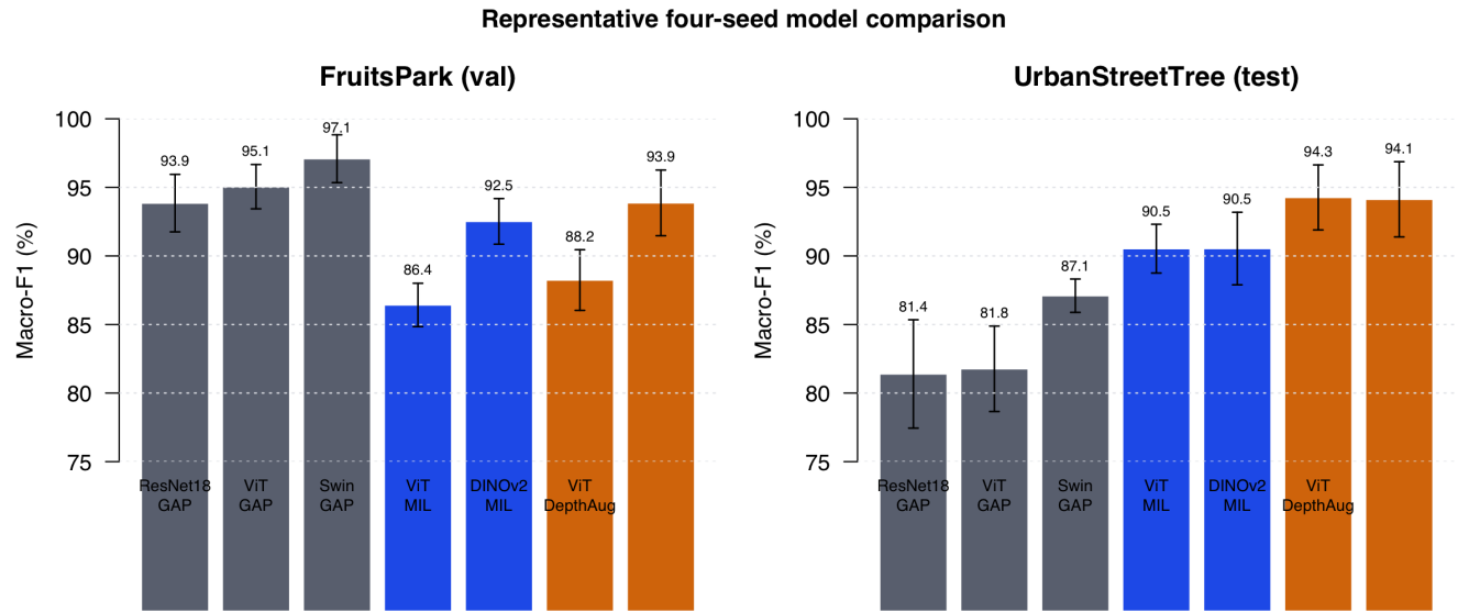
FIGURE 5. Representative four-seed macro- F_1 comparison. Gray bars indicate image-level GAP baselines, blue bars indicate sparse MIL, and orange bars indicate sparse MIL with DepthAug.
