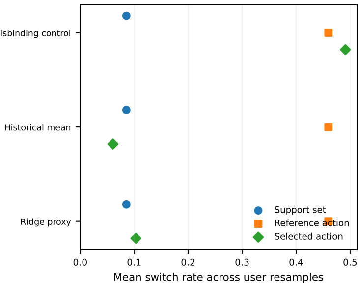
(b) Data-dependent selection instability
