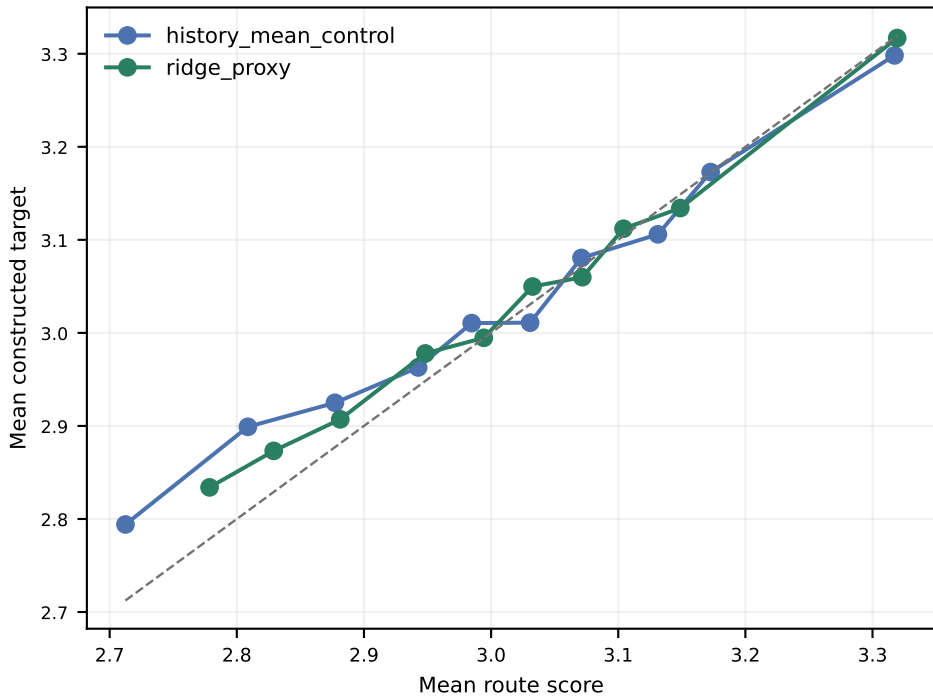
Score calibration by frozen decile
