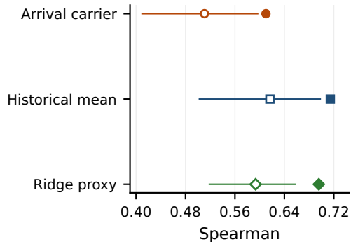
(a) Score recovery
