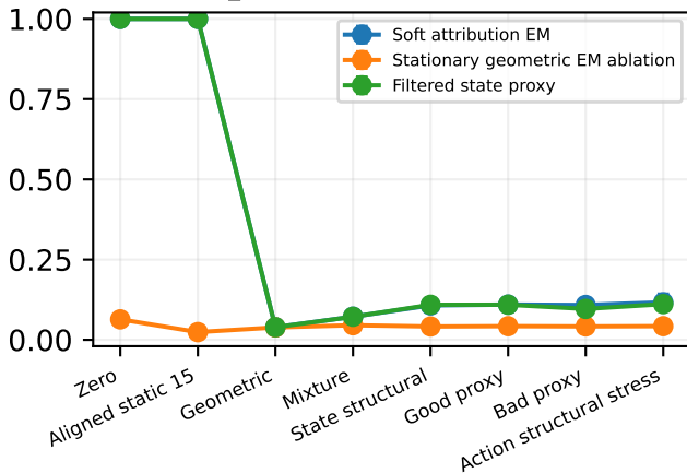
mixture_labelled: soft attribution true mass
