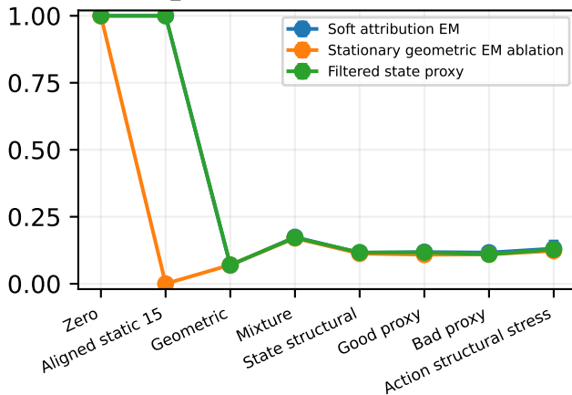
mixture_labelled: soft attribution top1 accuracy
