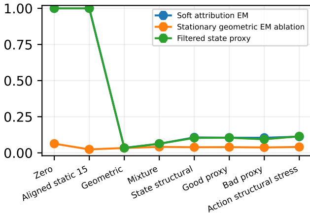
unlabelled: soft attribution true mass
