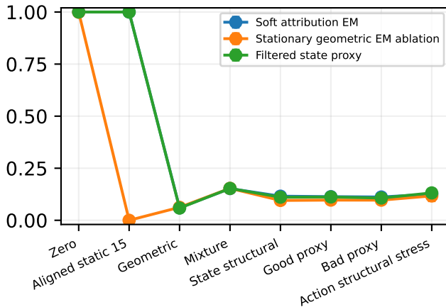
unlabelled: soft attribution top1 accuracy
