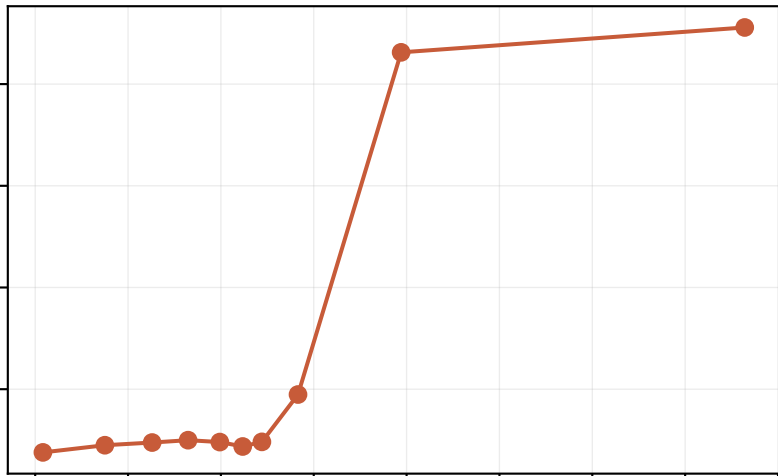
Mean ambiguity
