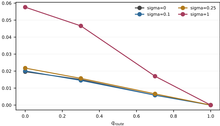
Optimal-set conflict rate
