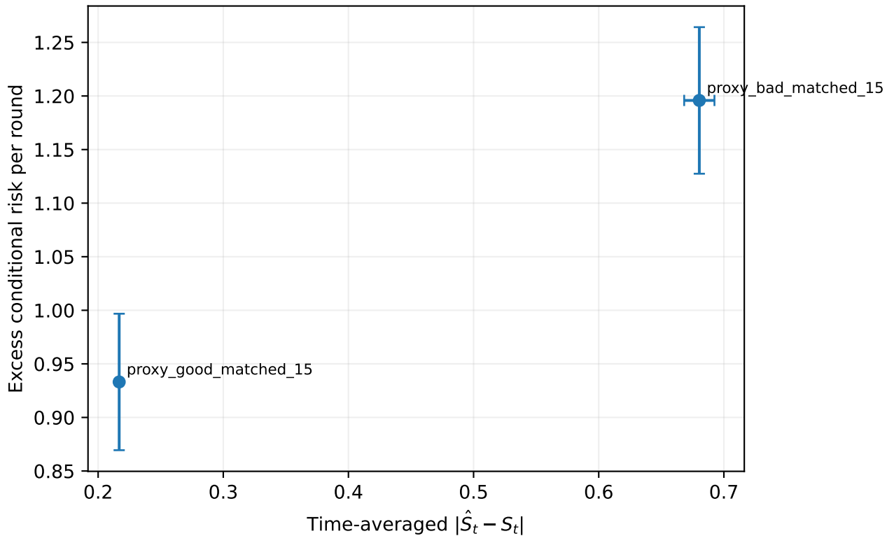
Proxy quality and regret (no source labels)
