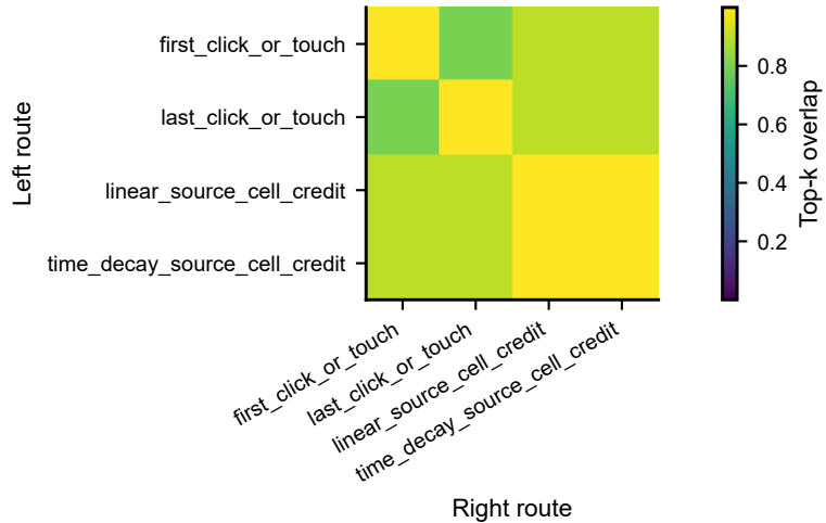
Pairwise Top-k diagnostics
