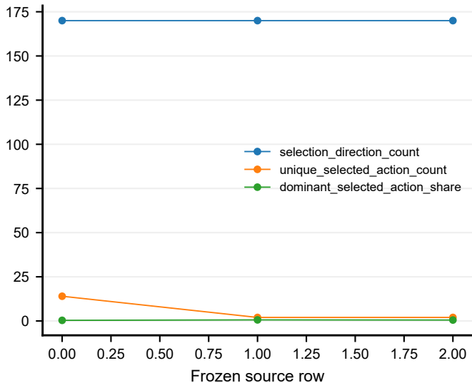
Route-selection concentration
