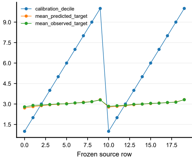
Decile calibration
