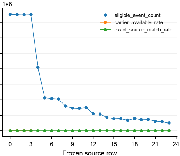
Arrival-carrier diagnostic
