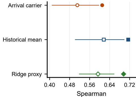
(a) Score recovery
