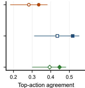
(c) Ranking recovery
