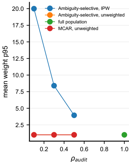
Weight diagnostics
