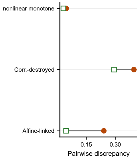
Control summary
