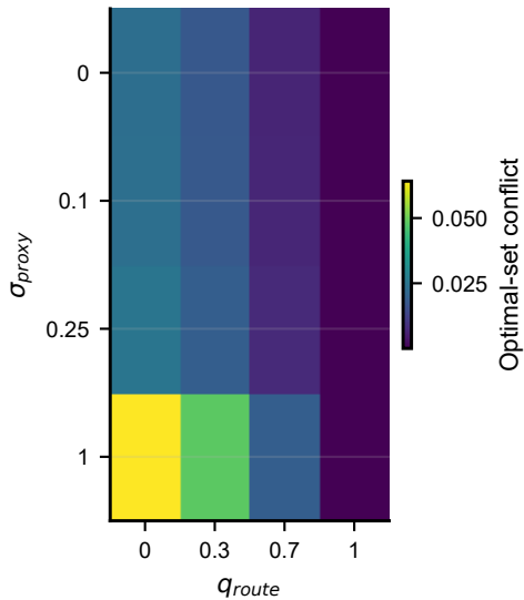
Conflict heatmap
