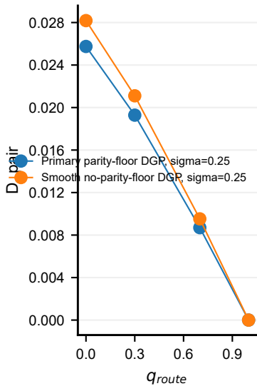
Loss robustness
