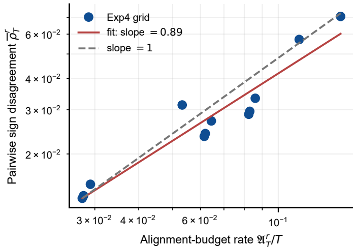
(b) Rate \bar{\rho}_T^r \sim (\mathfrak{A}_T^r/T)^{\kappa/(\kappa+1)}
