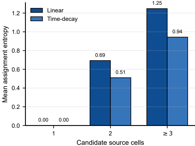
(a) Attribution entropy
