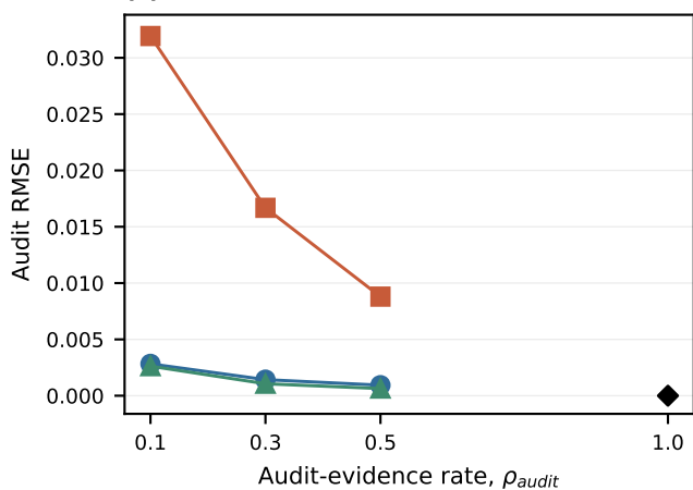
(c) Audit RMSE
