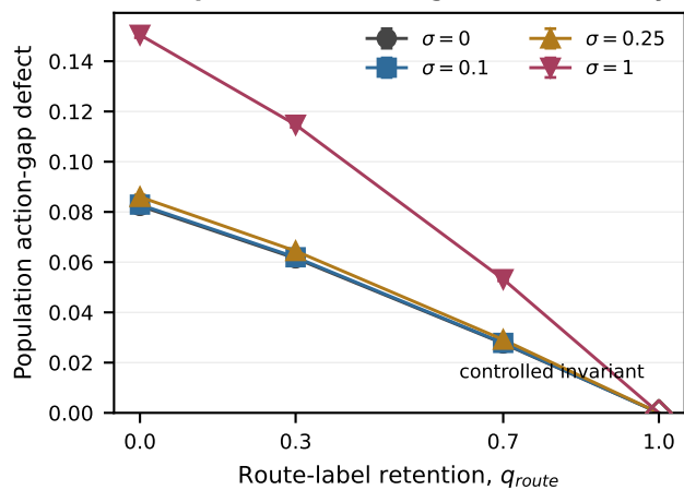
(a) Population route-alignment boundary
