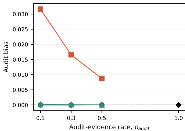
(b) Audit bias
