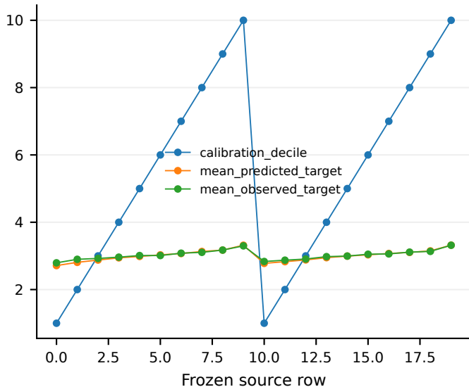
Decile Calibration
