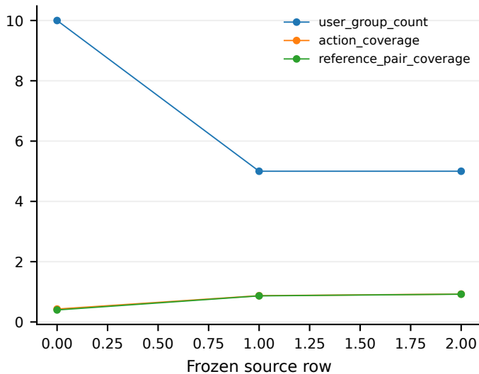
Full Design Support Preflight
