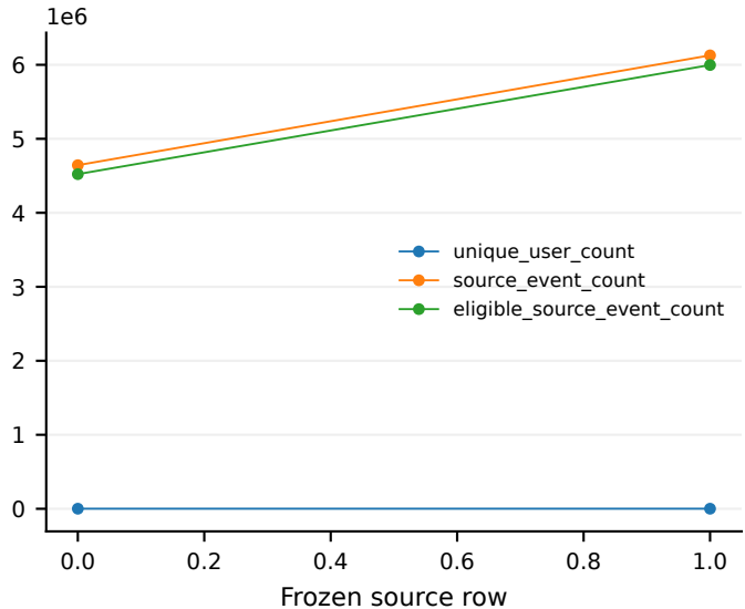
Data Dependence Structure
