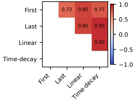
Kendall tau-b
