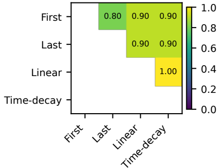
Top-10 overlap
