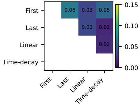
Allocation TV
