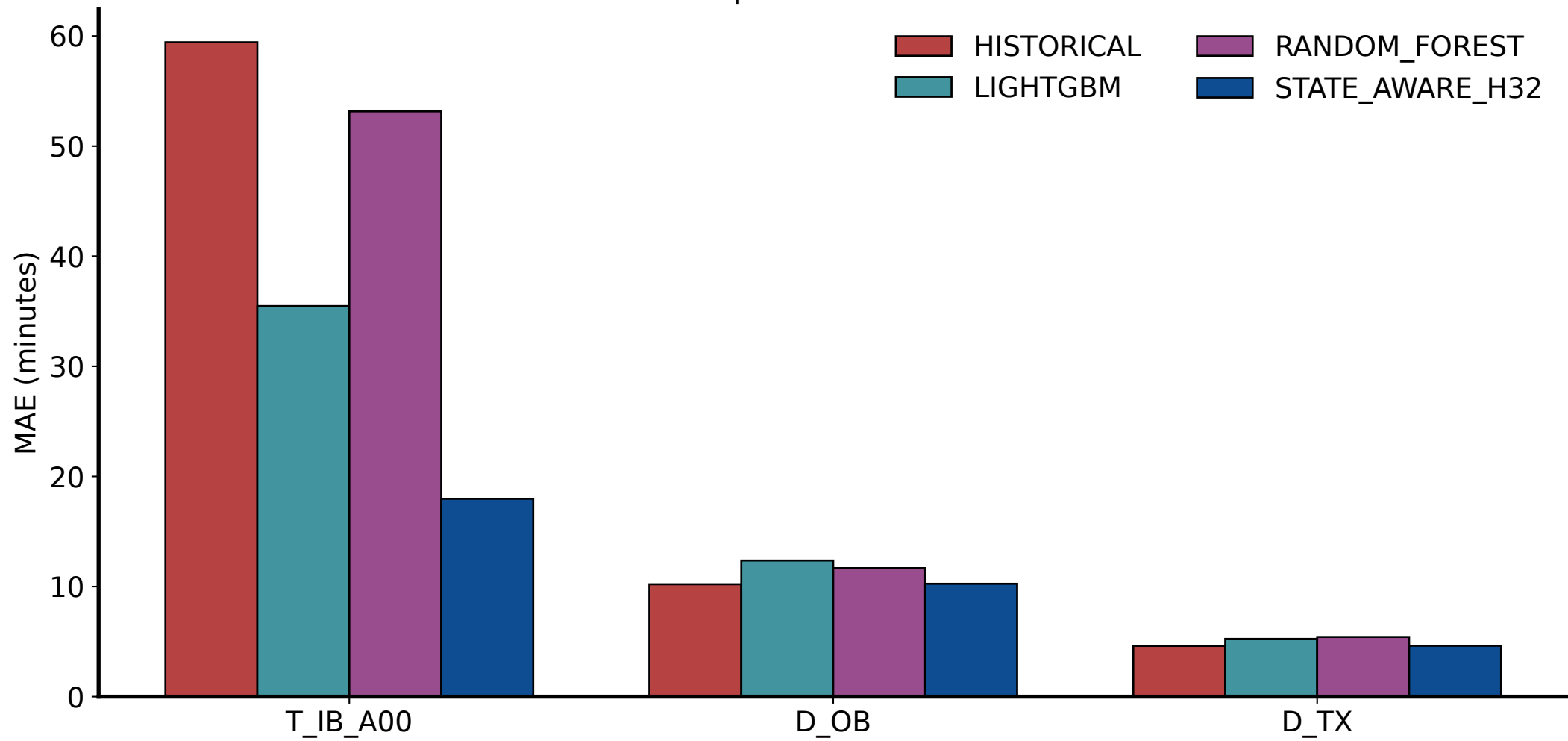
Final Test predictive benchmark
